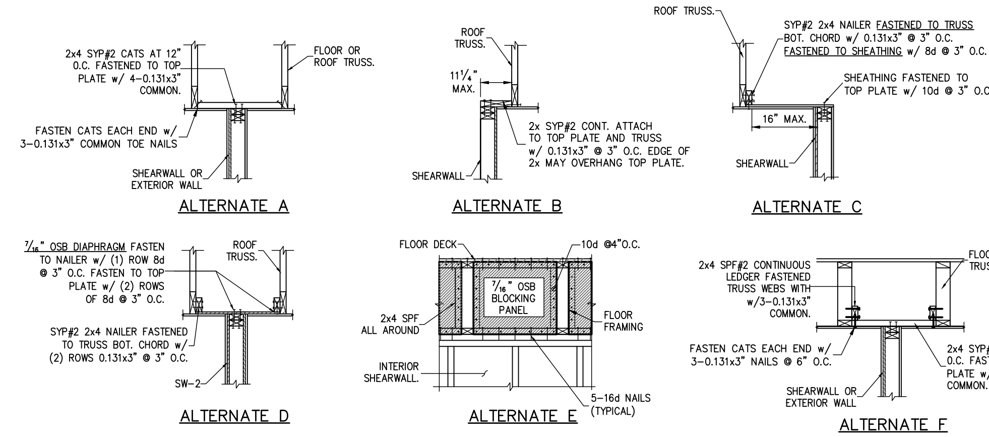
5 SHEARWALL ATTACHMENT AT ROOF & FLOOR S.O.1
