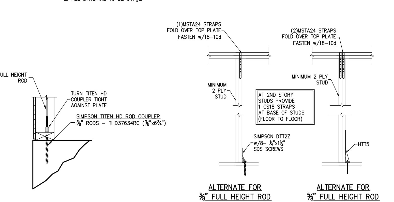
13 3/8" FULL HEIGHT ROD ALTERNATE ATTACHMENT S.O.1
