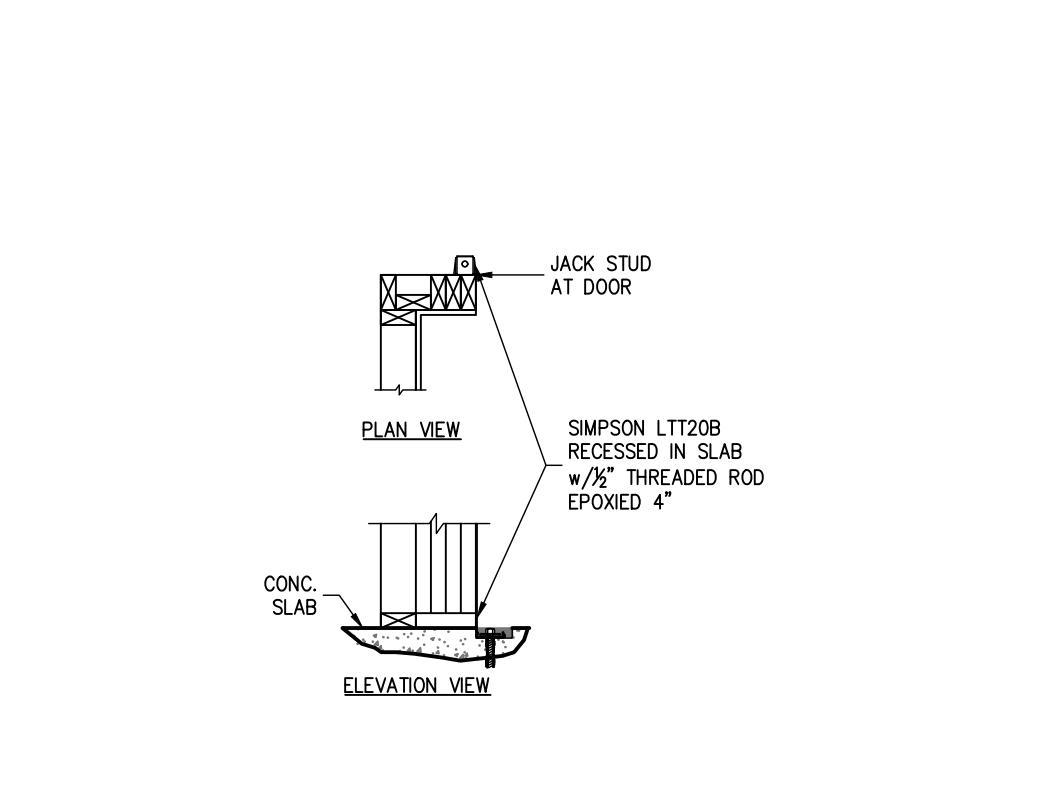
16 DOOR JAMB FASTENING S.O.1 WHEN NOTED THIS DETAIL ONLY APPLIES WHEN NOTED ON PLAN
