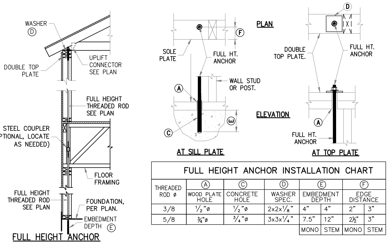
12 FULL HEIGHT WOOD FRAME WALL ANCHORING SYSTEM S.O.1 THIS DETAIL ONLY APPLIES WHEN NOTED ON PLAN
