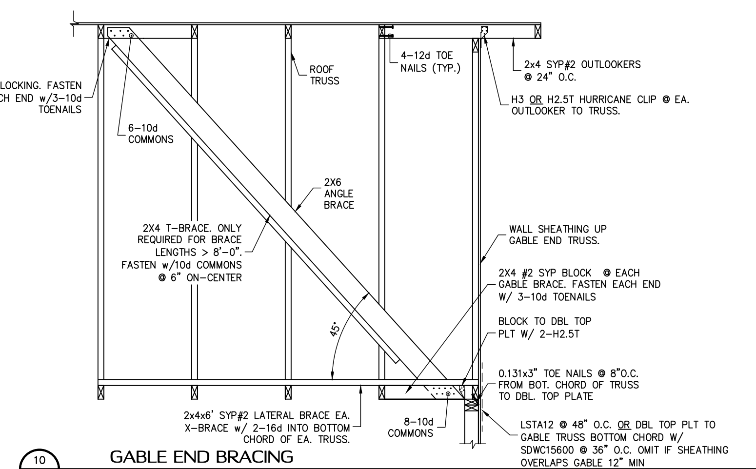
10 GABLE END BRACING S.O.1 NOTES: 1. SPACE GABLE END BRACING @ 4'-6" MAX. 2. ALL MATERIAL TO BE SYP#2
