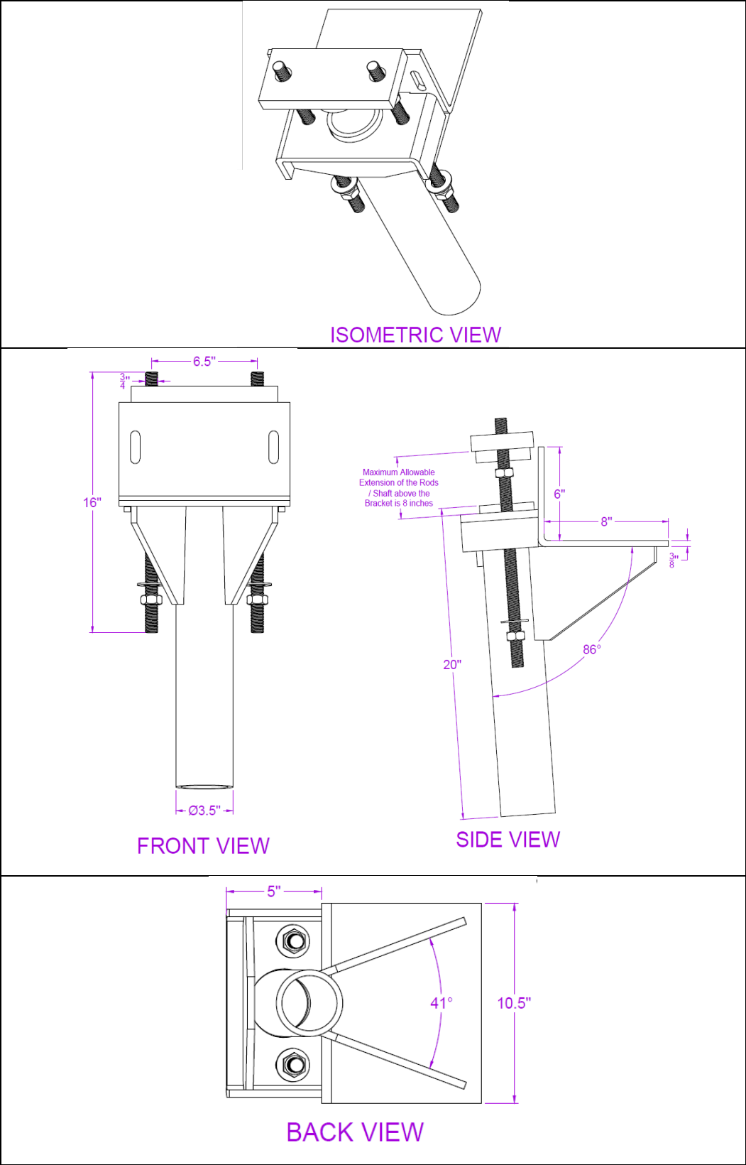
FIGURE 3—UNDERPINNING BRACKET
