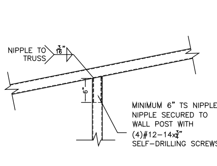
ROOF PANEL CONNECTION VERTICAL SHEATHING OPTION
