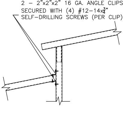
LEAN-TO TO TRUSS CONNECTION
