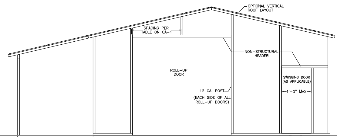
TYPICAL END ELEVATION
