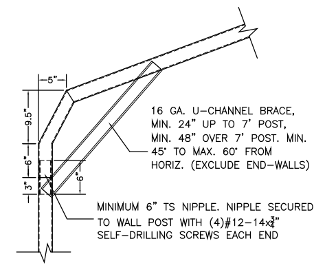
BOW RAFTER TO POST CONNECTION DETAIL
