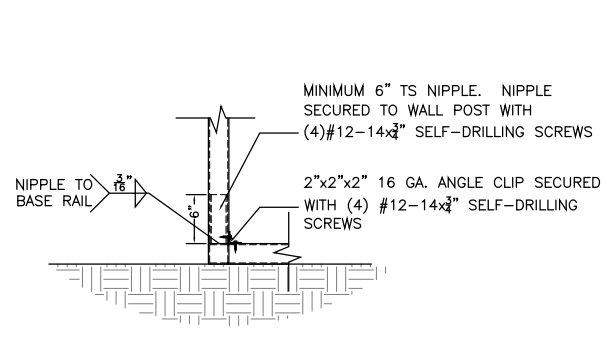
END POST TO BASE RAIL CONNECTION
