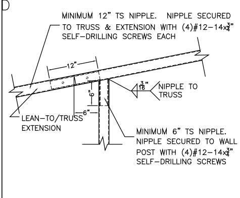
LEAN-TO TO TRUSS CONNECTION
