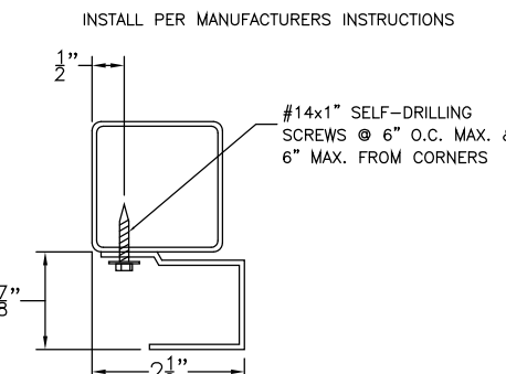
END POST TO BASE RAIL CONNECTION
