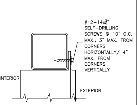
DOOR FRAME TO POST CONNECTION
