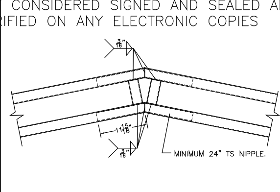
TRUSSED RAFTER CONNECTION DETAIL
