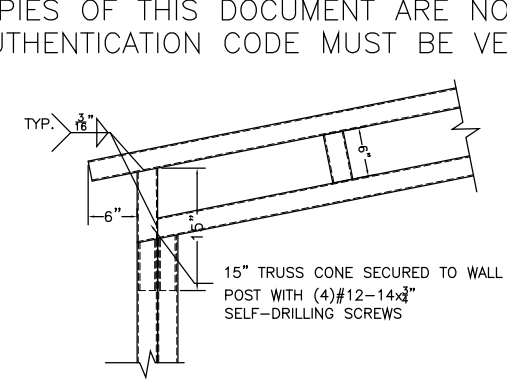
40' BOX EAVE RAFTER TO POST CONNECTION DETAIL
