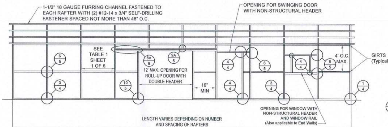
TYPICAL POST/RAFTER/GIRT FRAMING PLAN (12' WIDE MAX. OPENING) NOT TO SCALE
