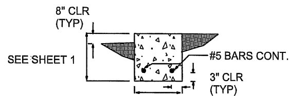
RIBBON FOOTING
