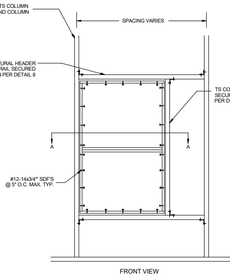
11 WINDOW INSTALLATION DETAILS N.T.S.
