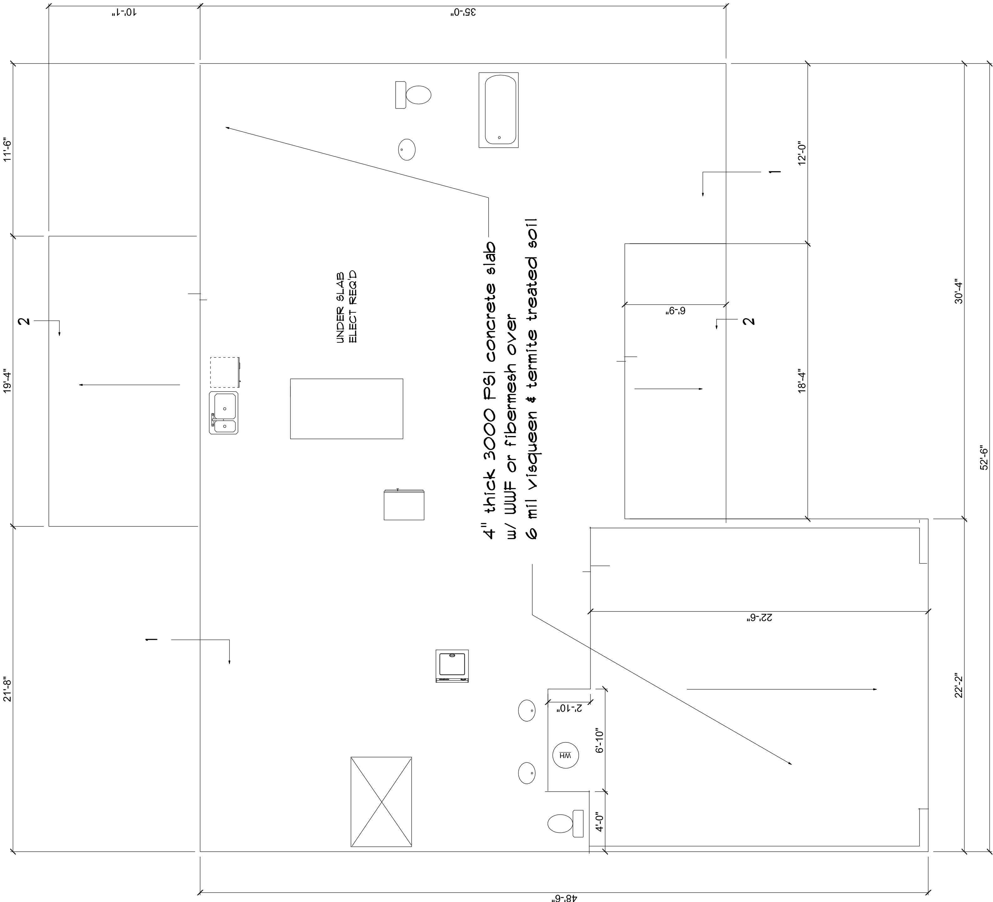
FOUNDATION PLAN
