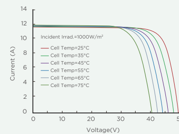
Current-Voltage Curve(SP440M-72HB)
