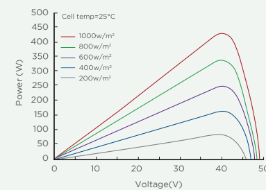
Current-Voltage Curve(SP440M-72HB)
