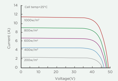
Current-Voltage Curve(SP440M-72HB)
