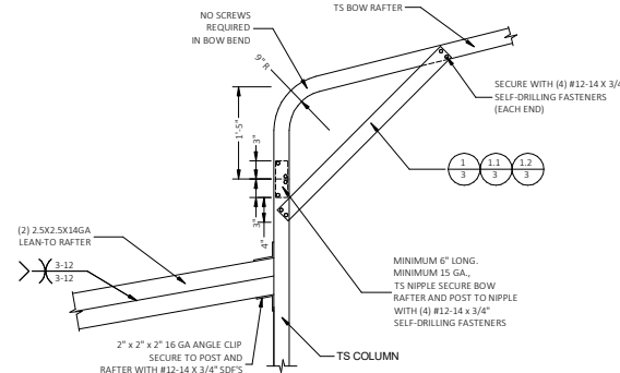
SIDE EXTENSION RAFTER/COLUMN DETAIL FOR EXTENSION RAFTER SPANS 16'-0" < W' < 24'-0" , IF THE KNEE BRACE ON THE OTHER END OF THE RAFTER IS PER DETAIL 1.2/3. FOR EXTENSION RAFTER SPANS 18'-0" < W' < 24'-0" , IF THE KNEE BRACE ON THE OTHER END OF THE RAFTER IS PER DETAIL 1.1/3. FOR EXTENSION RAFTER SPANS 19'-0" < W' < 24'-0" , IF THE KNEE BRACE ON THE OTHER END OF THE RAFTER IS PER DETAIL 1/3. SCALE: NTS
