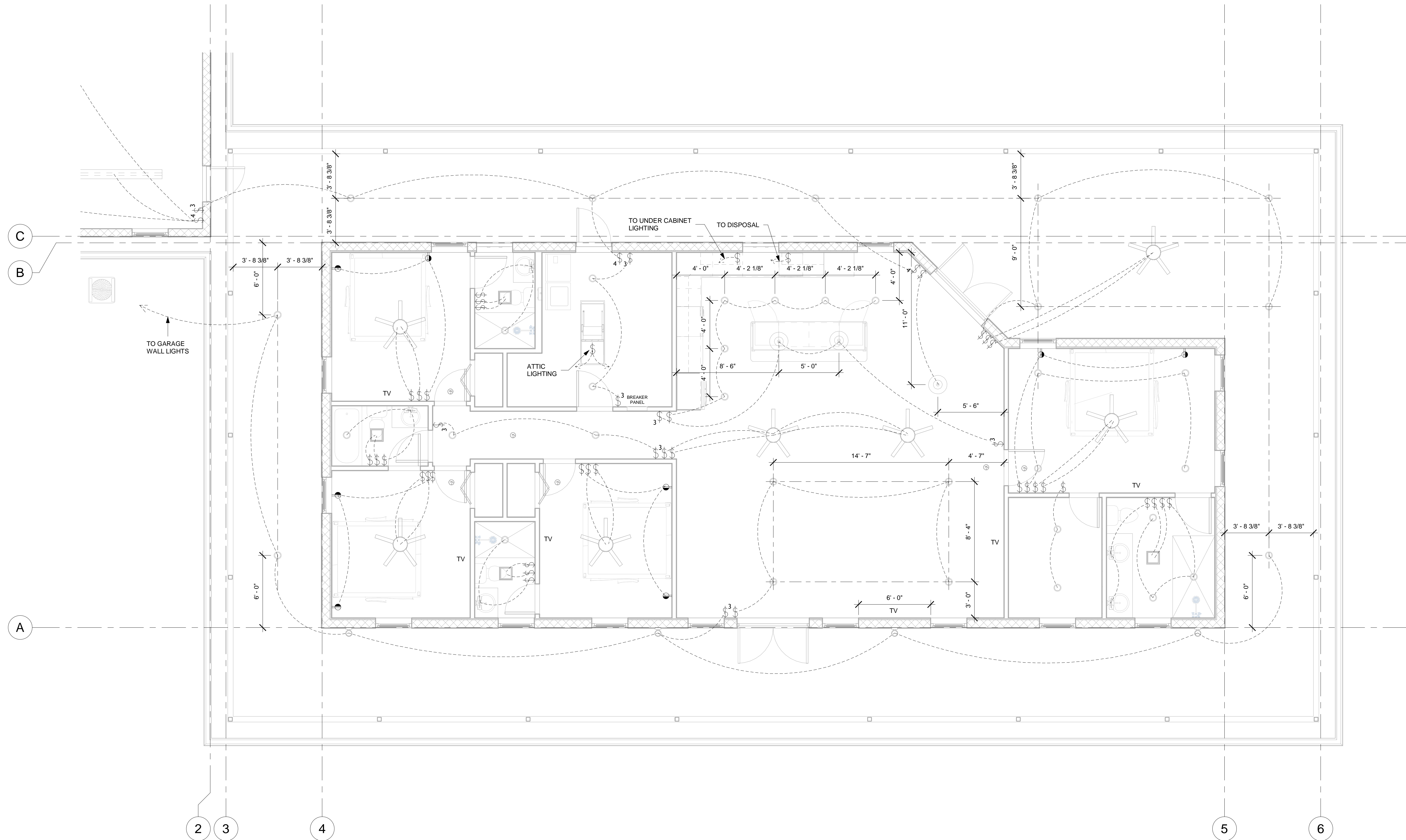
1 Lighting Plan 1/4" = 1'-0"
