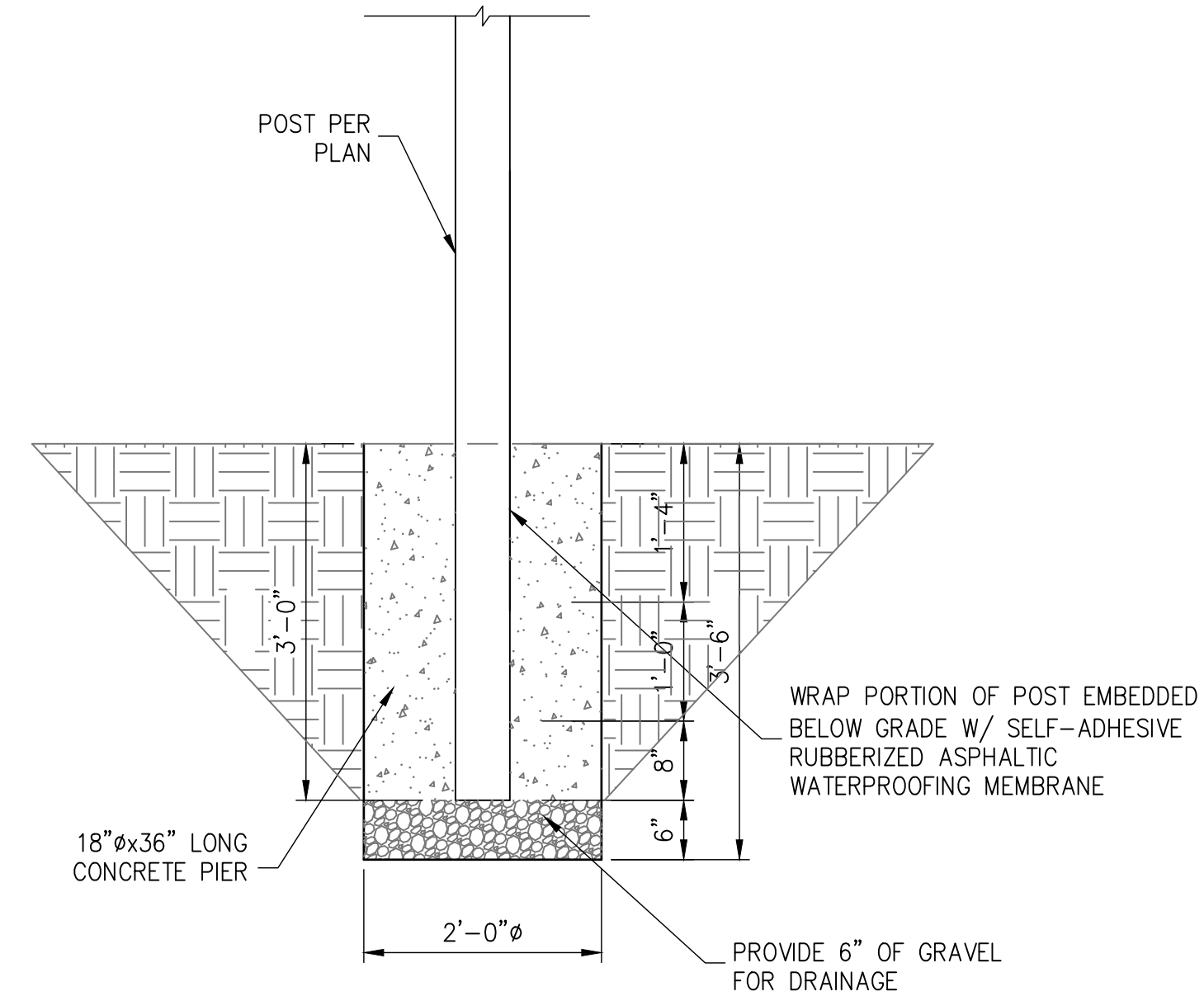
10 EMBEDDED POST DETAIL S1.01 SCALE: 3/4" = 1'-0"
