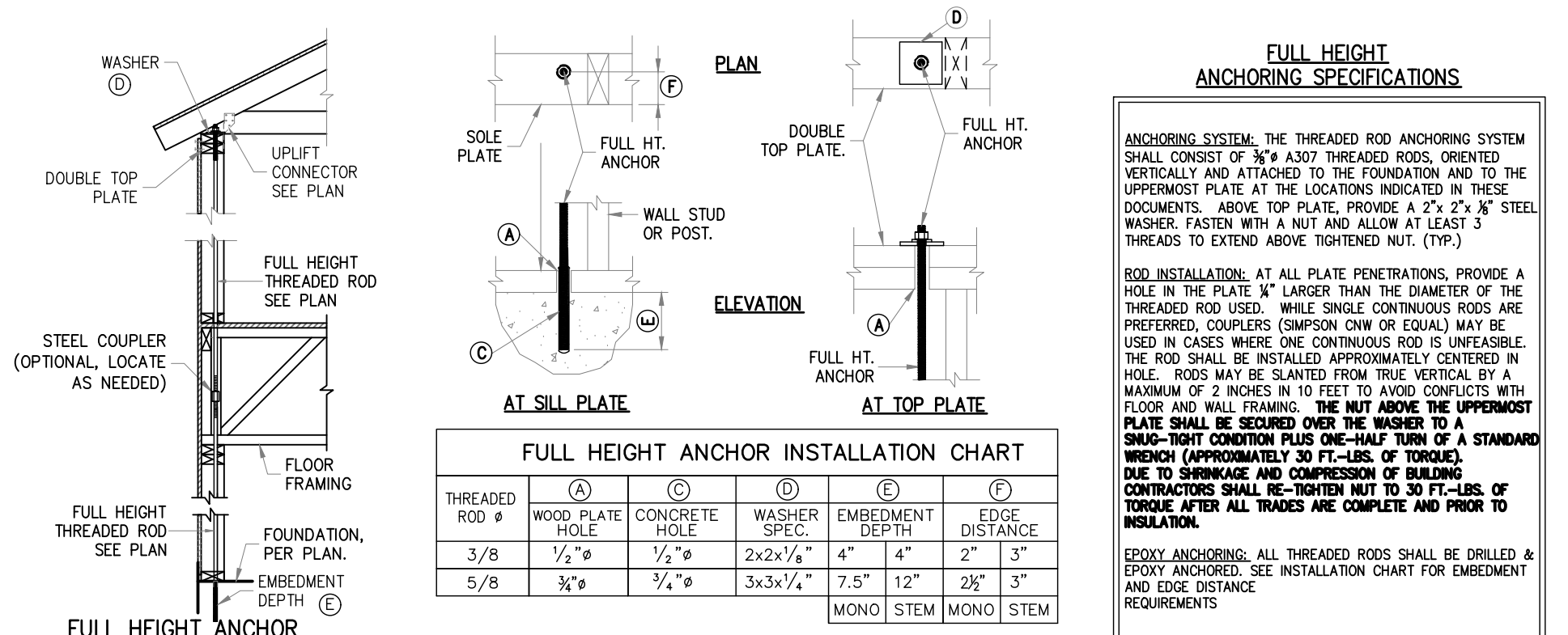
12 FULL HEIGHT WOOD FRAME WALL ANCHORING SYSTEM S.O.1 THIS DETAIL ONLY APPLIES WHEN NOTED ON PLAN
