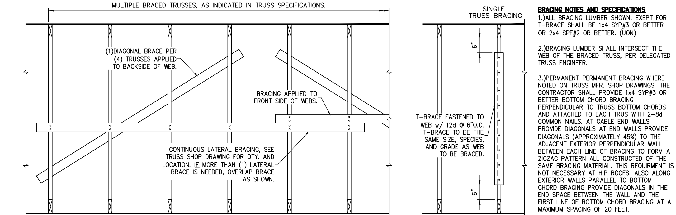
11 PERMANENT TRUSS BRACING S.O.1 SCALE: 3/4" = 1'-0"
