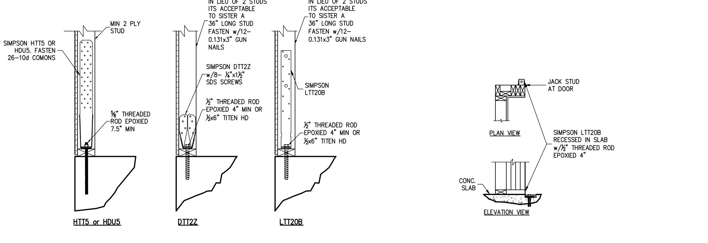
15 HOLD DOWN ATTACHMENT DETAIL S.O.1
