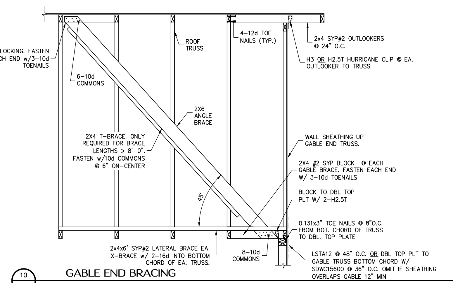
10 GABLE END BRACING S.O.1 NOTES: 1. SPACE GABLE END BRACING @ 4'-6" MAX. 2. ALL MATERIAL TO BE SYP#2
