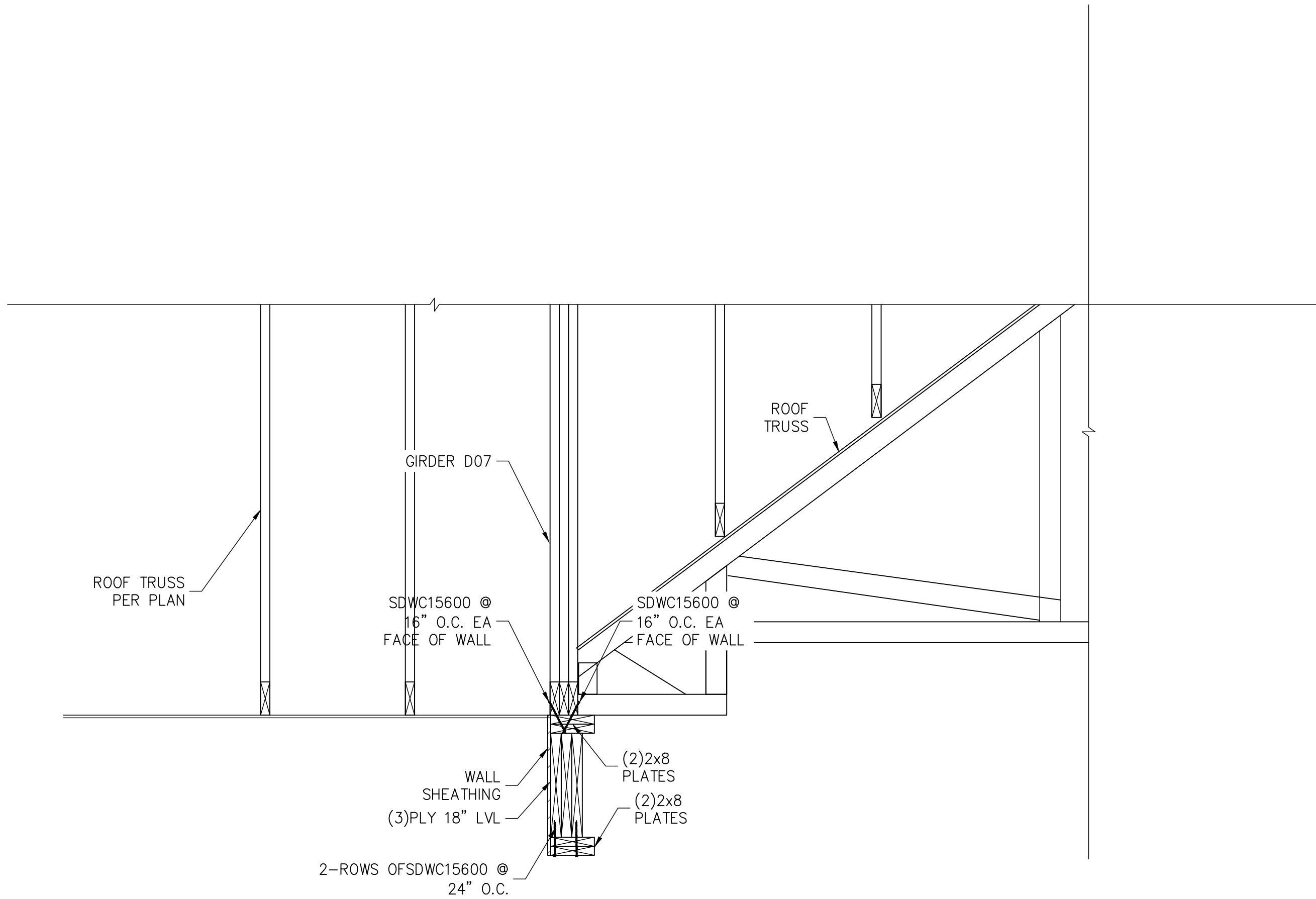
2 ROOF SECTION AT SGD S2.1 SCALE: 3/8"=1'-0"
