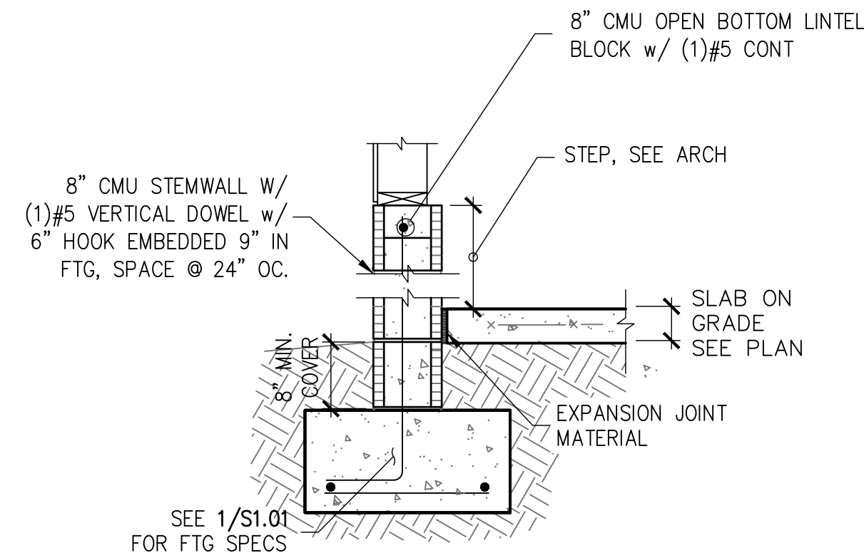
7 GARAGE PERMETER STEMWALL WITH FLOATING SLAB S1.01 SCALE: 3/4" = 1'-0"
