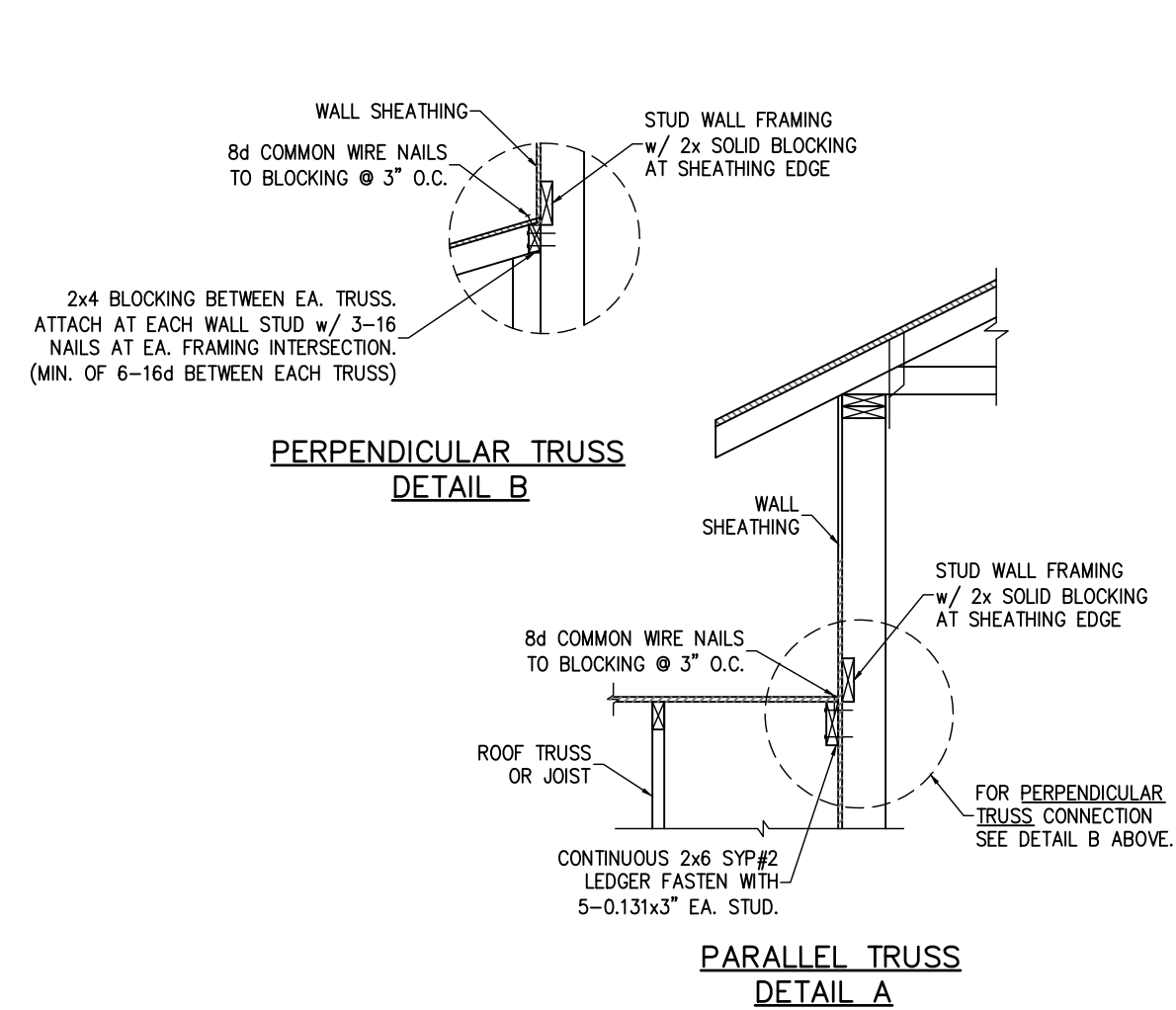
4 WALL ADJ. TO ROOF CONNECTION S.O.1 WHEN NOTED SEE CONSTRUCTION SPECIFICATIONS FOR ROOF AND WALL SHEATHING AND STUD FRAMING.
