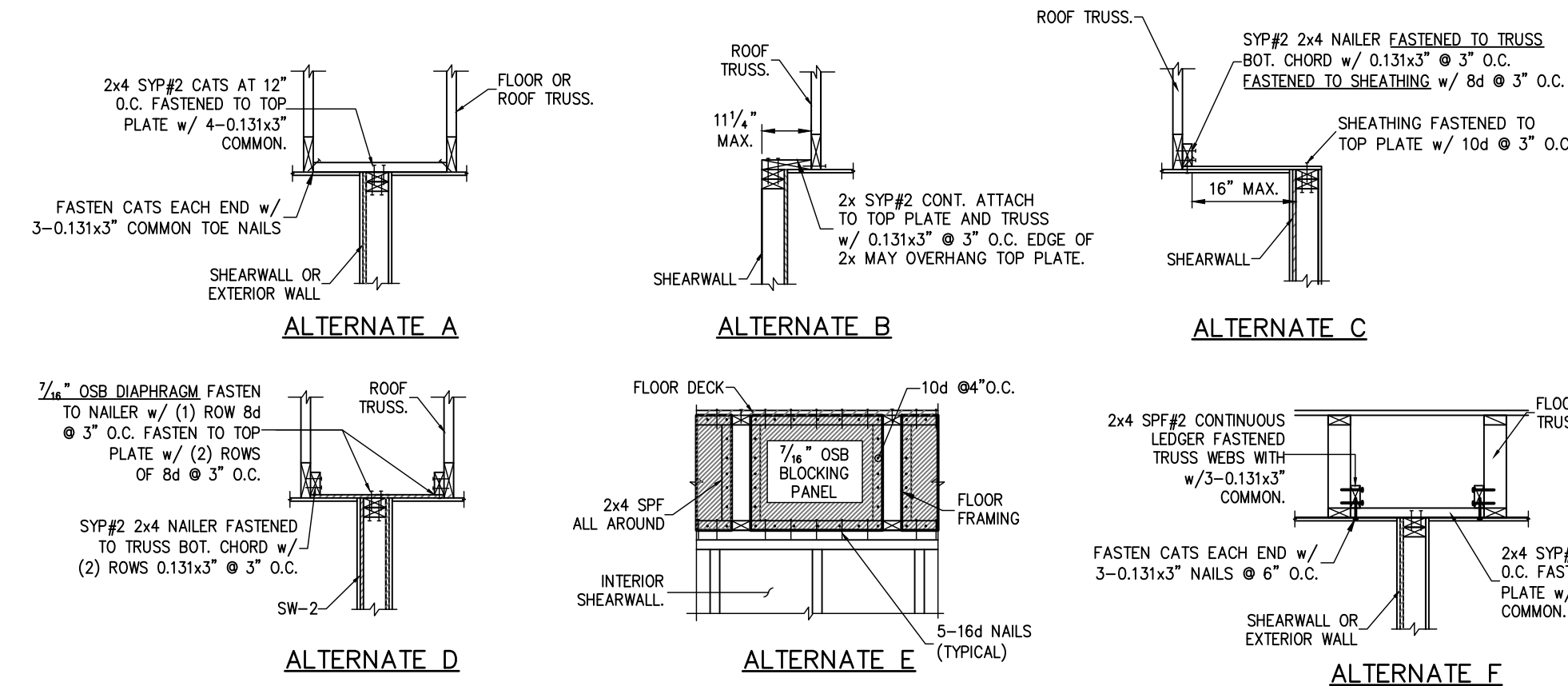
5 SHEARWALL ATTACHMENT AT ROOF & FLOOR S.O.1
