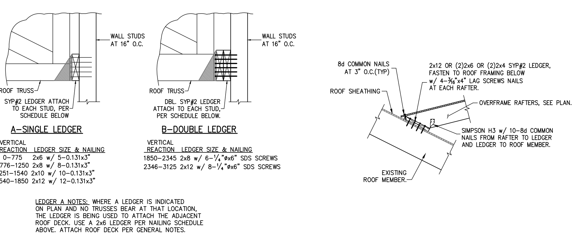
8 LEDGER CONNECTION S.O.1 TRUSS TO LEDGER CONNECTION BY TRUSS ENGINEER, NOT SHOWN FOR CLARITY
