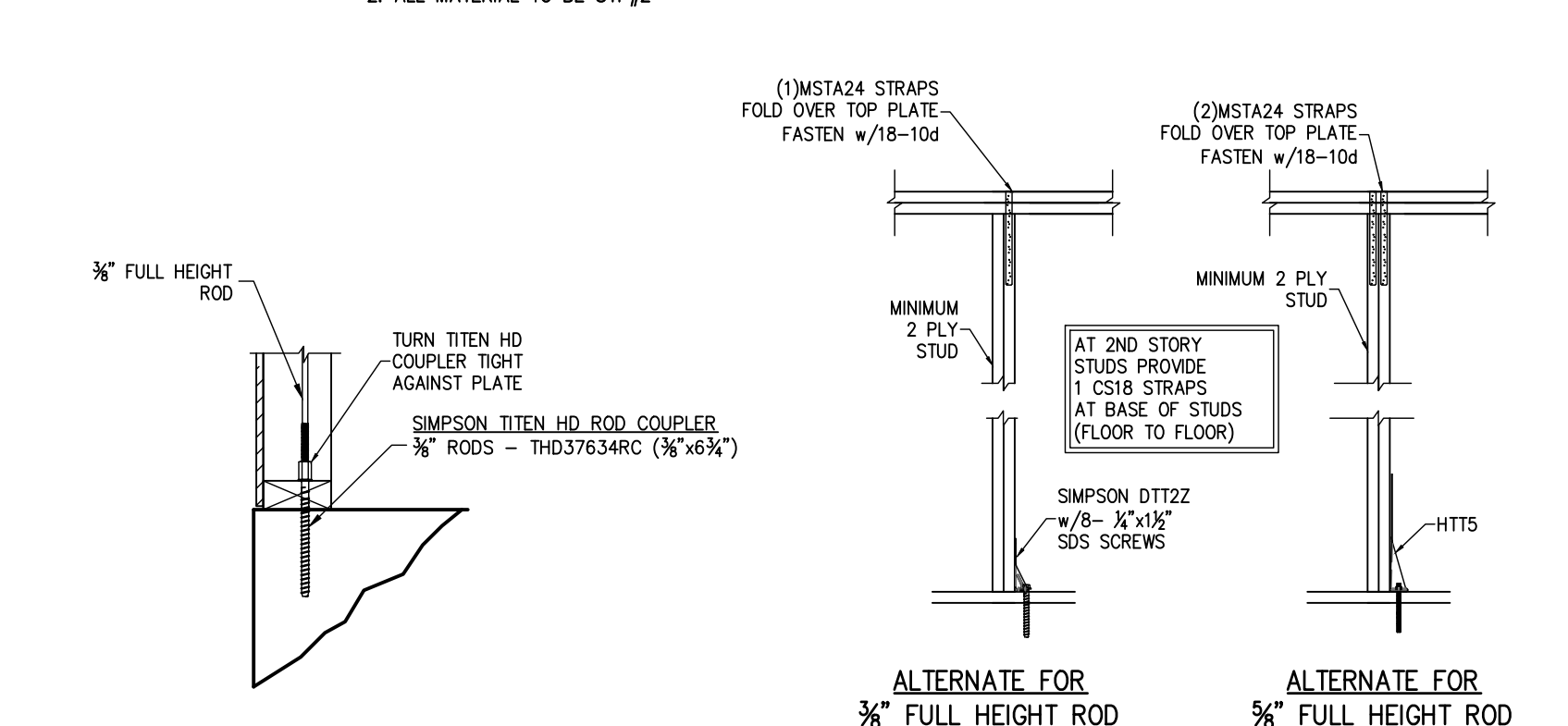
13 3/8" FULL HEIGHT ROD ALTERNATE ATTACHMENT S.O.1
