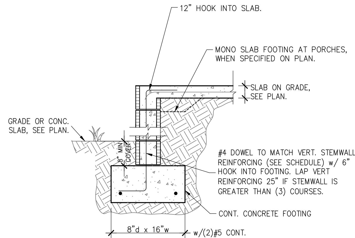
9 STEMWALL AT LANAI AND PORCH S1.01 SCALE: 3/4" = 1'-0"
