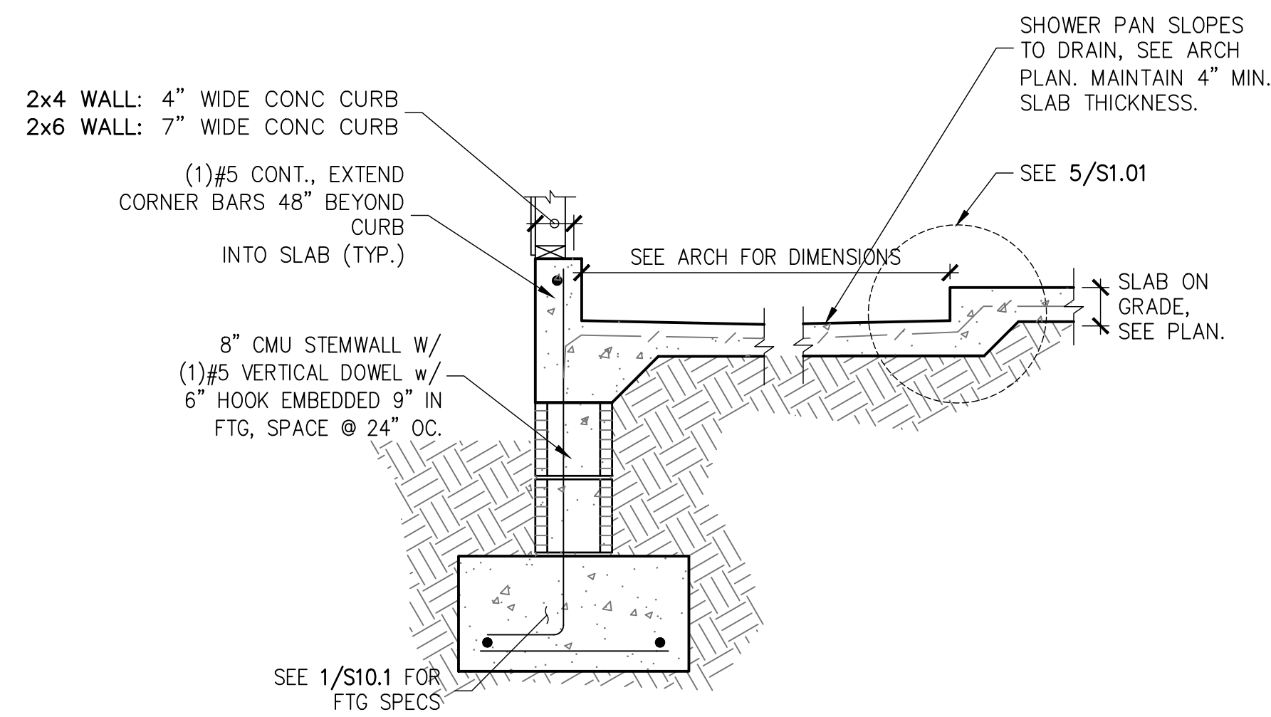
8 SHOWER CURB AT EDGE WALL S1.01 SCALE: 3/4" = 1'-0"
