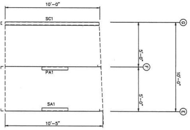
PARTITION WALL FRAMING FRAME LINE: 4 (Typ of 22) GRID LINES: (4-24)
