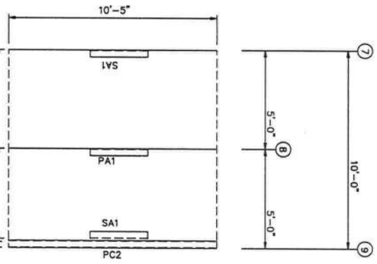
PARTITION WALL FRAMING FRAME LINE: E (Typ of 3) GRID LINES: (23-25)(39-41)
