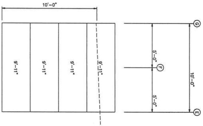
PARTITION WALL SHEETING FRAME LINE: 4 (Typ of 22) GRID LINES: (4-24) PANELS: 29 Ga. PBR - Galvalume
