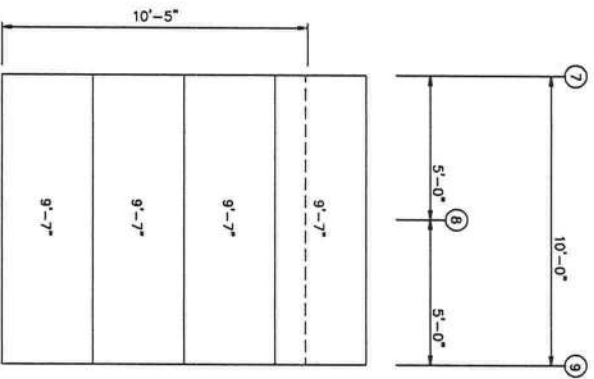
PARTITION WALL SHEETING FRAME LINE: E (Typ of 3) GRID LINES: (23-25)(39-41) PANELS: 29 Ga. PBR - Galvalume
