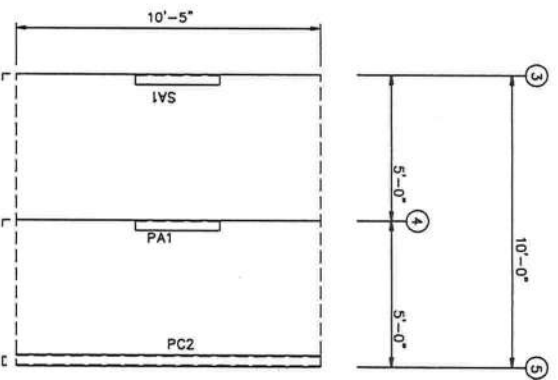
PARTITION WALL FRAMING FRAME LINE: E (Typ of 23) GRID LINES: (3-55)
