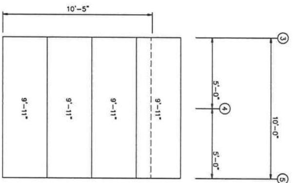
PARTITION WALL SHEETING FRAME LINE: E (Typ of 23) GRID LINES: (3-55) PANELS: 29 Ga. PBR - Galvalume
