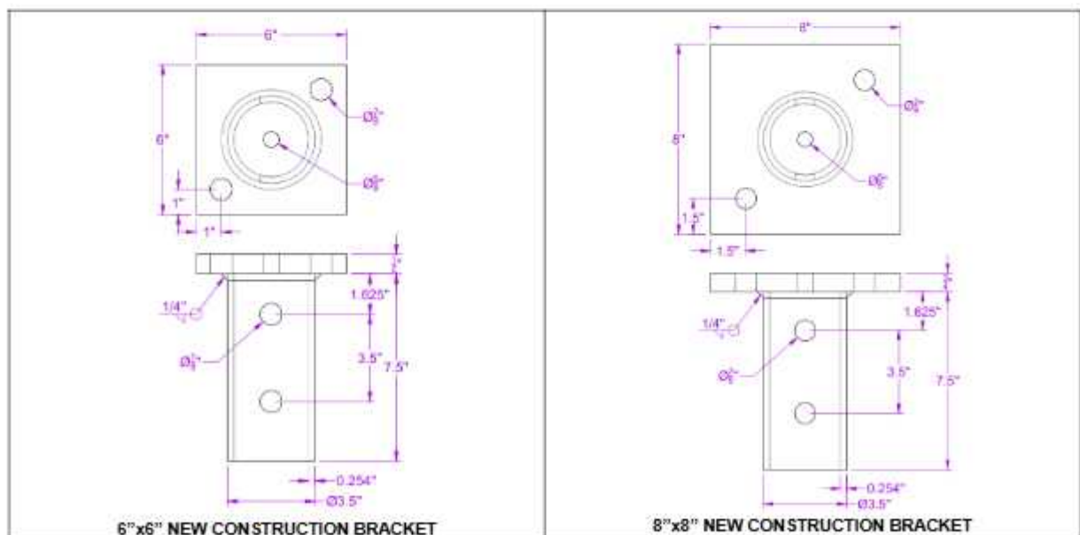
FIGURE 2—NEW CONSTRUCTION BRACKET
