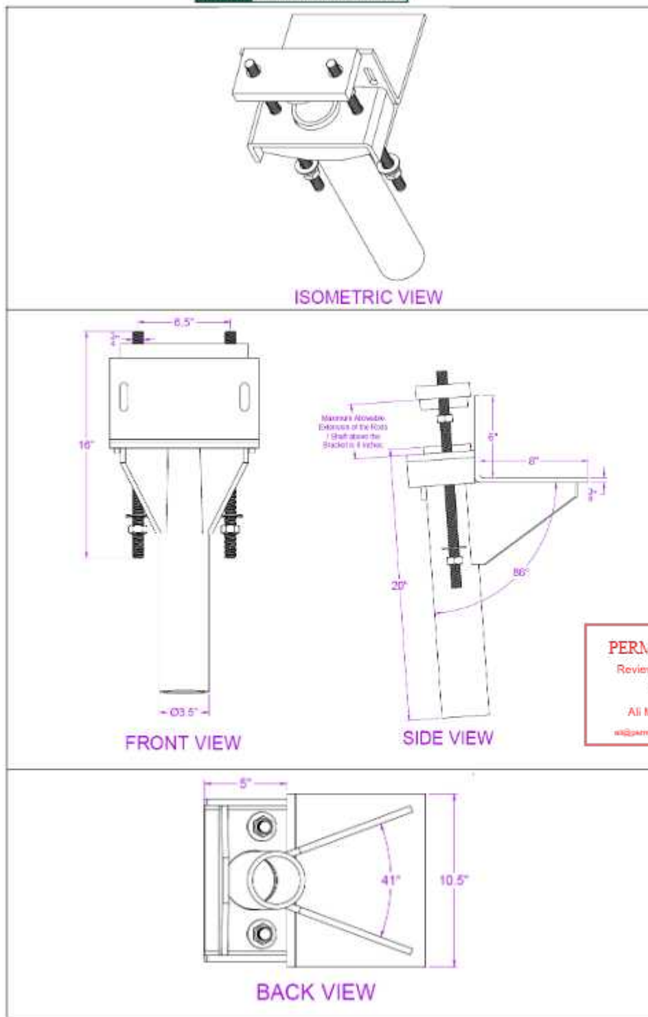
FIGURE 3—UNDERPINNING BRACKET
