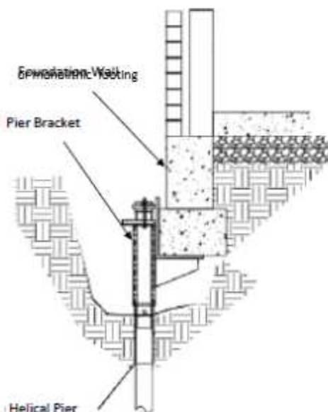
Helical Pier/Bracket Detail (Typ.)
