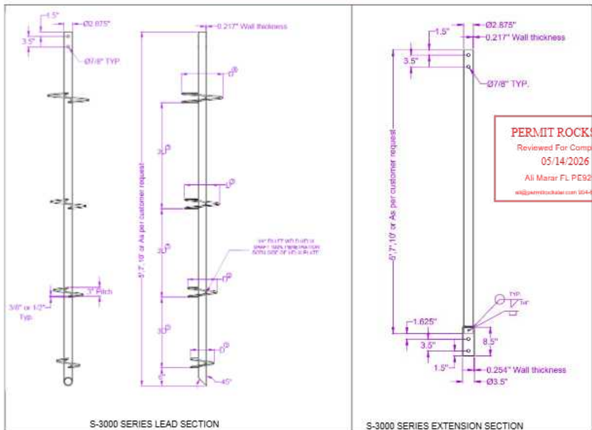
FIGURE 1—S-3000 SERIES LEAD AND EXTENSION SECTIONS
