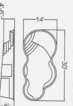
AXIOM 14/NEBULA - CRUL 8,000 gal. approx.
