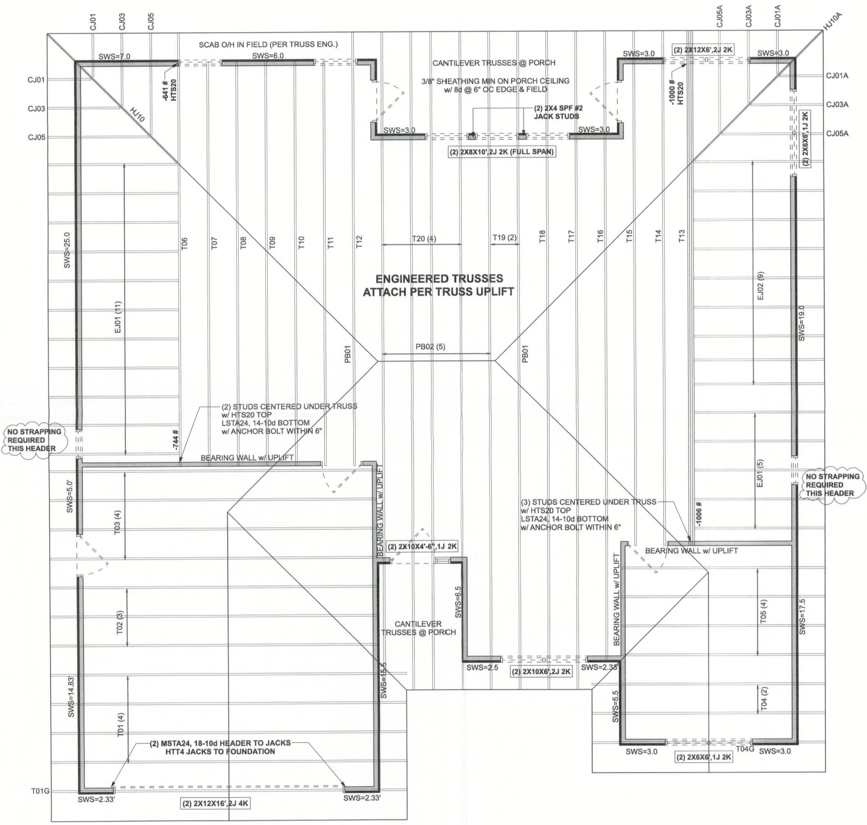
STRUCTURAL PLAN SCALE: 1/4" = 1'-0"
