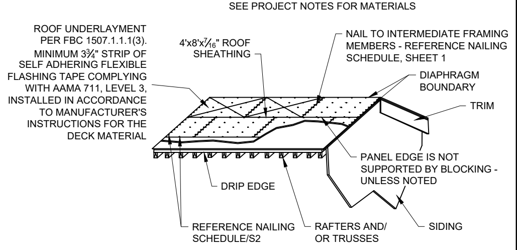
3 ROOF SHEATHING AND UNDERLAYMENT DETAIL SCALE: N.T.S.
