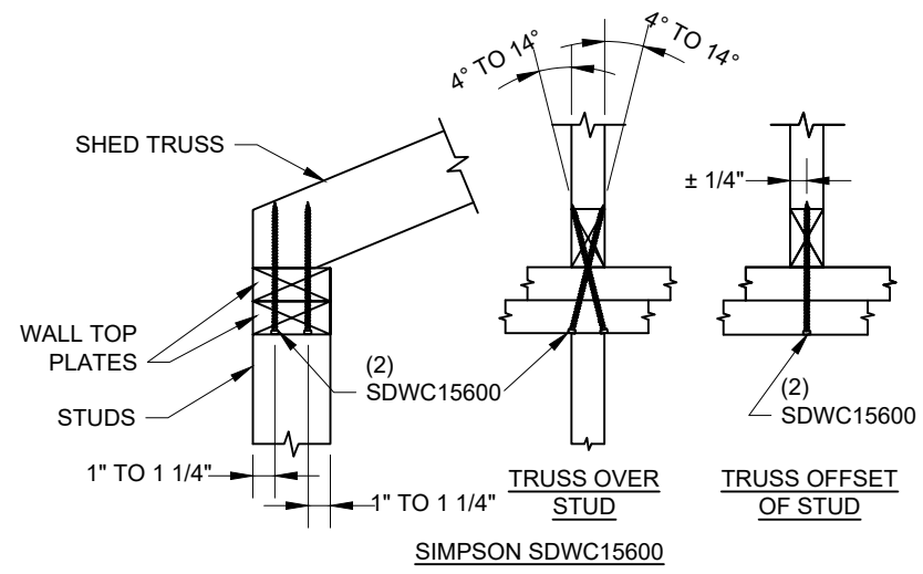
2 TRUSS TO WALL CONNECTION DETAIL SCALE: N.T.S.
