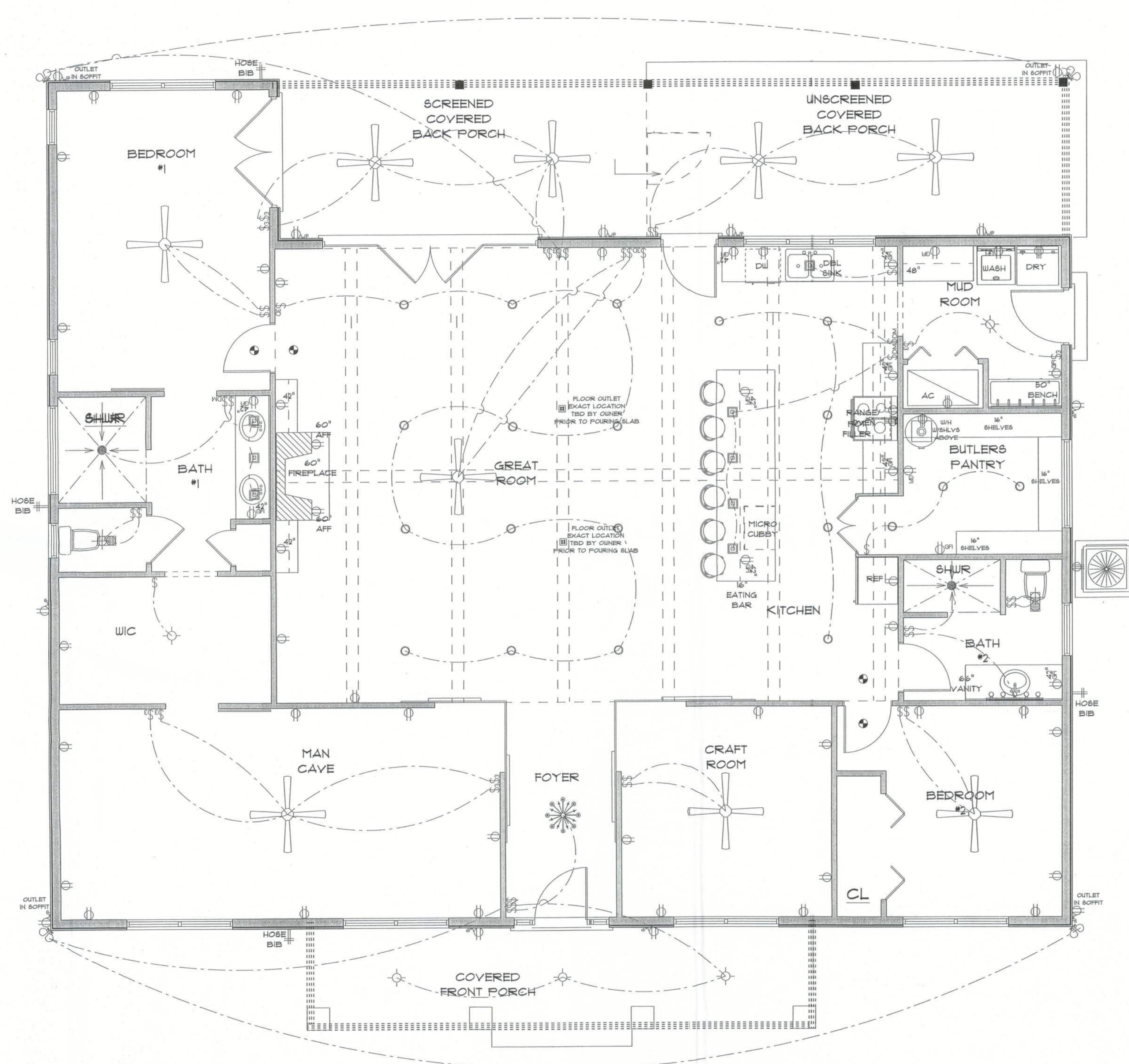
* ELECTRIC PLAN * SCALE : 1/4" = 1'-0"
