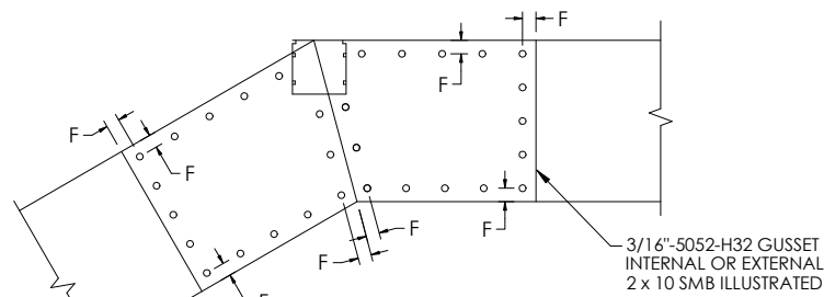
DETAIL "H" BEAM TO GUTTER CONNECTION SCALE: NTS
