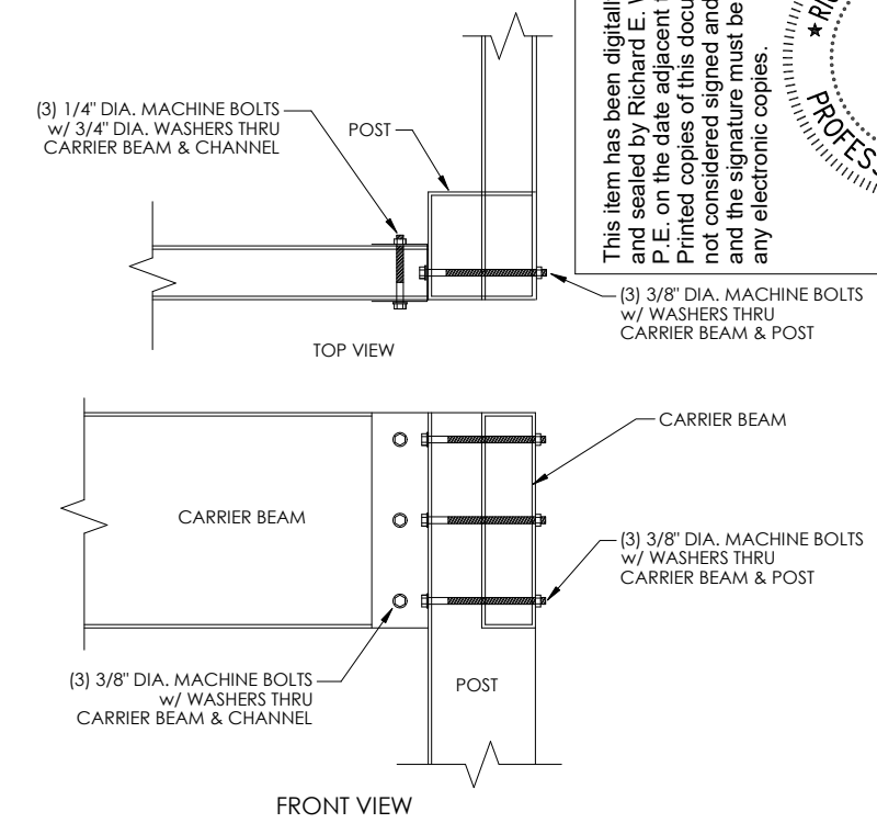
CORNER CARRIER BEAM CONNECTION DETAIL SCALE: NTS
