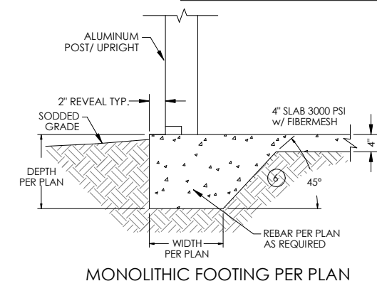
DETAIL "J" REVEAL SCALE: NTS
