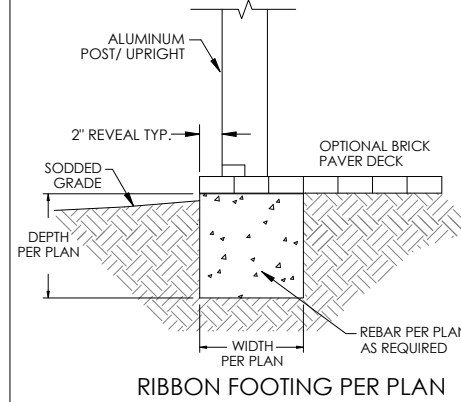
DETAIL "J" REVEAL SCALE: NTS
