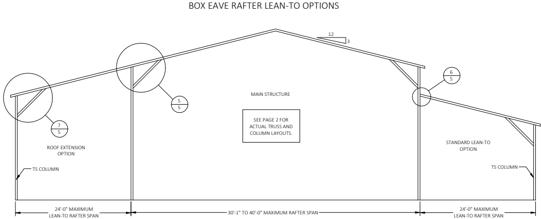
TYPICAL BOX EAVE RAFTER LEAN-TO OPTIONS FRAMING SECTION (BOTH OPTIONS SHOWN)
