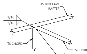
4 TRUSS POST AND CHORD TO RAFTER CONNECTION SCALE: NTS
