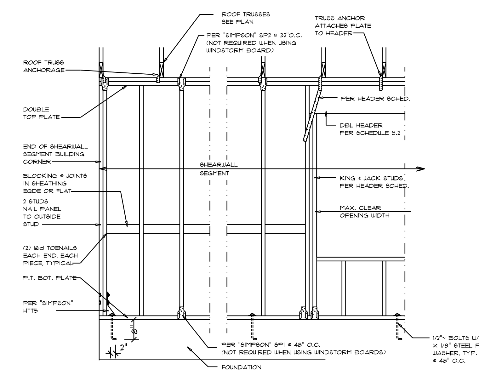
Shear Wall DETAILS SCALE: NONE
