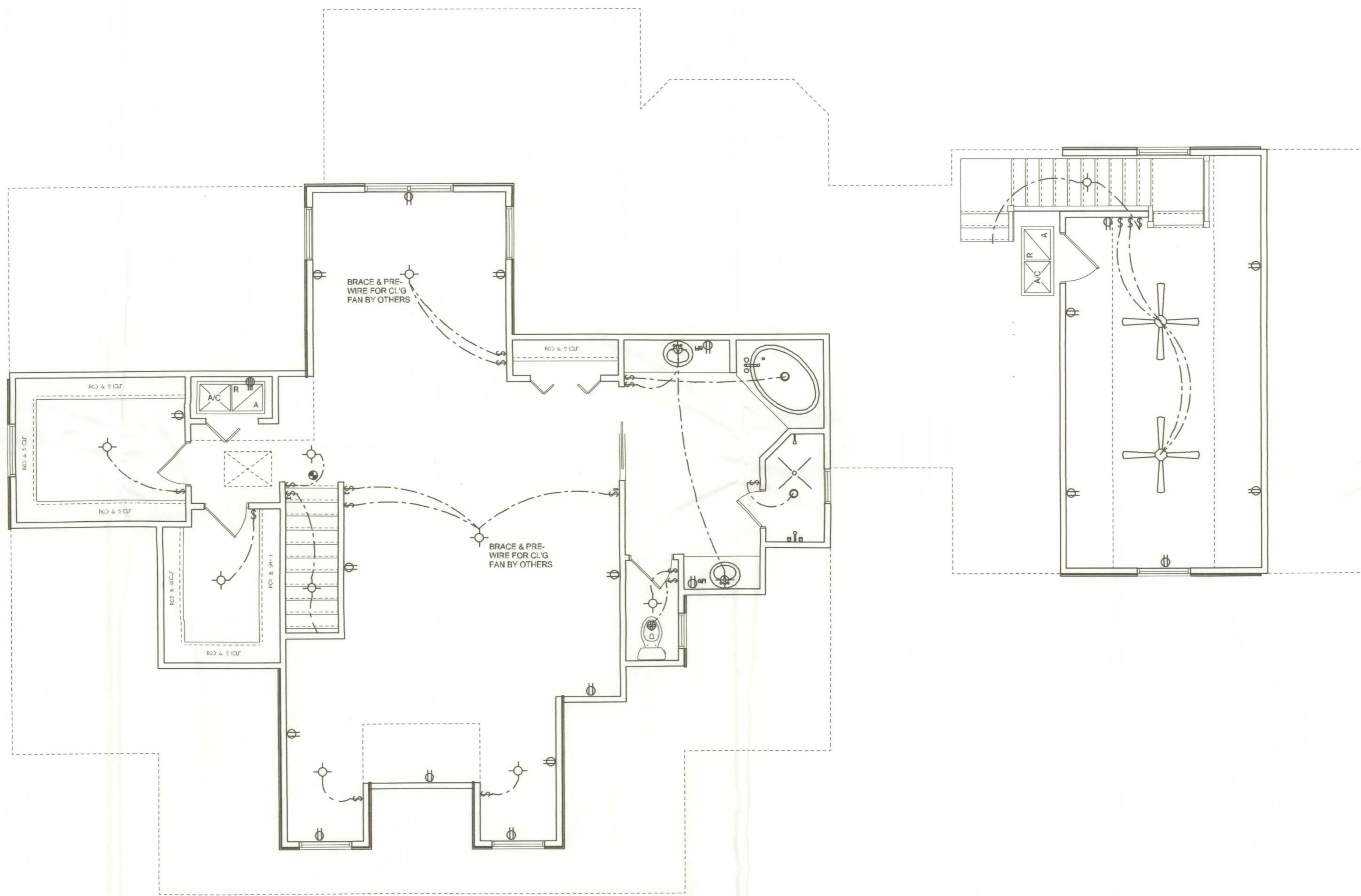
2nd FLOOR ELECTRICAL PLAN SCALE: 1/4" = 1'-0"
