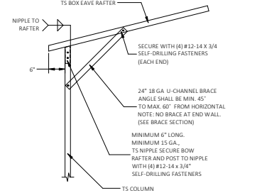
1.2 BOX EAVE RAFTER COLUMN CONNECTION DETAIL FOR HEIGHTS 12'-0" < TO <= 13'-0" SCALE: NTS
