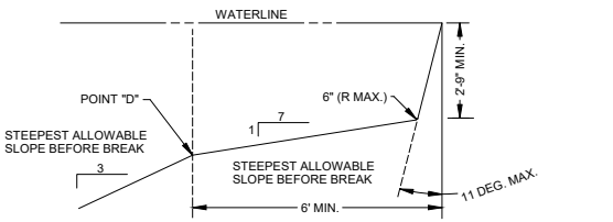
ALLOWABLE POOL FLOOR & WALL GEOMETRY
