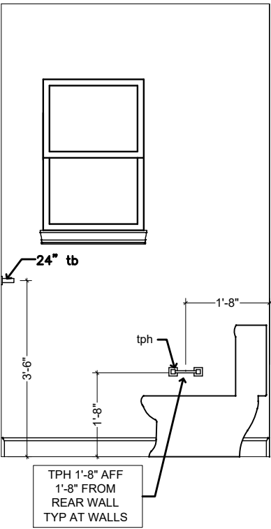
wall "W" powder bath
