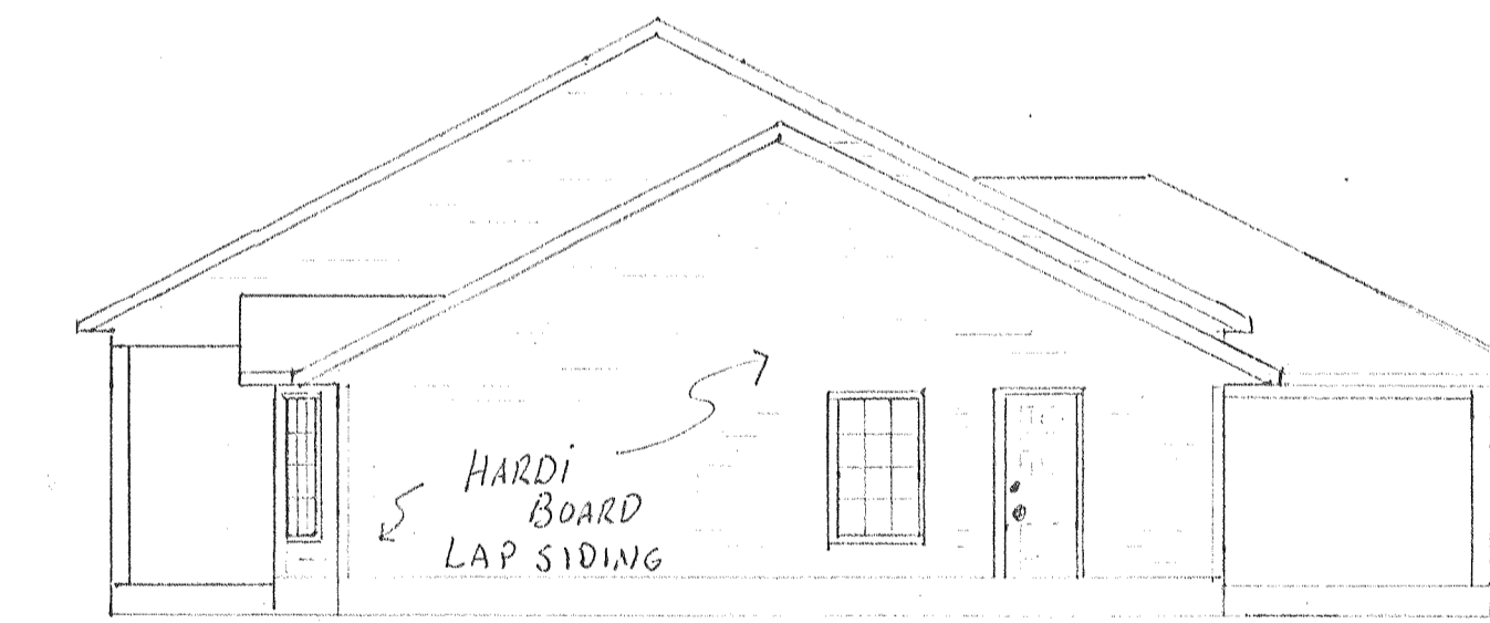
RIGHT SIDE ELEVATION 1" = 1/8"
