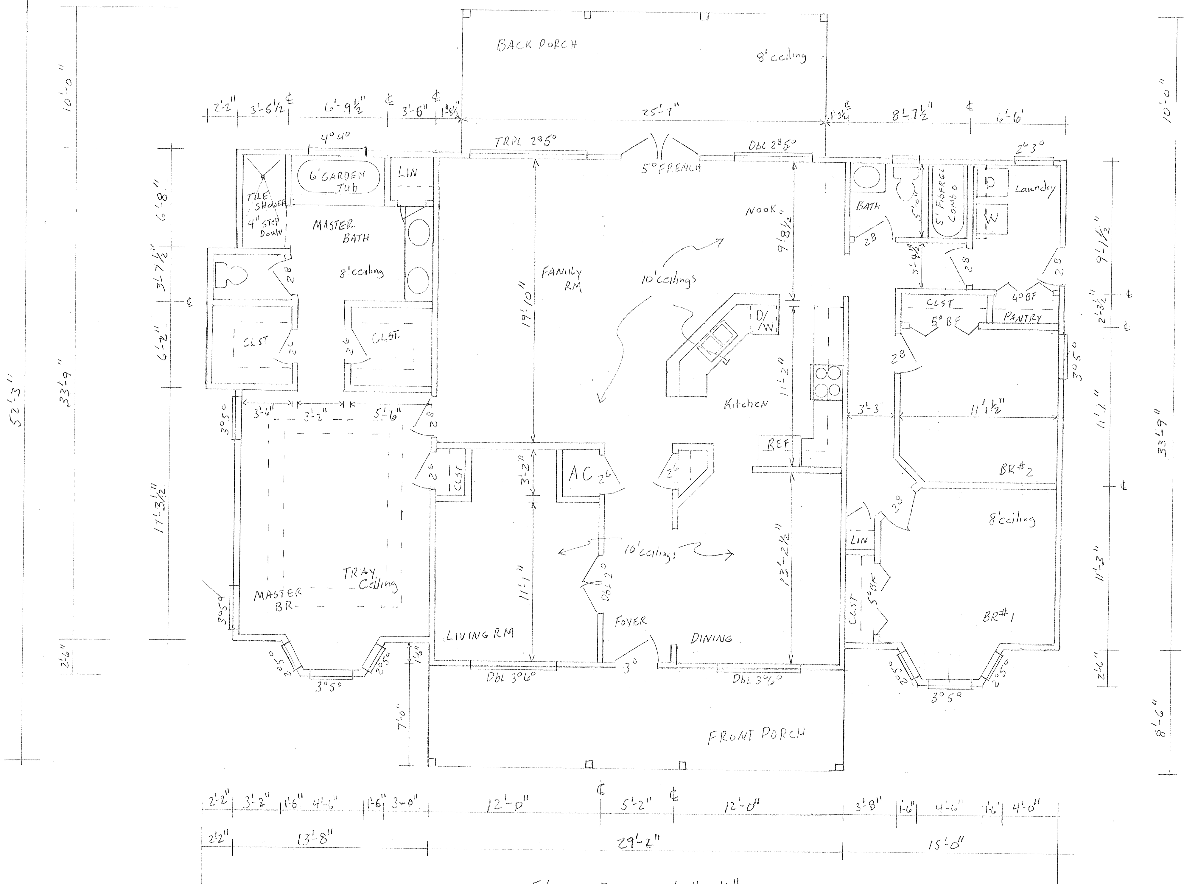
FLOOR PLAN 1'-0" = 1/4"
