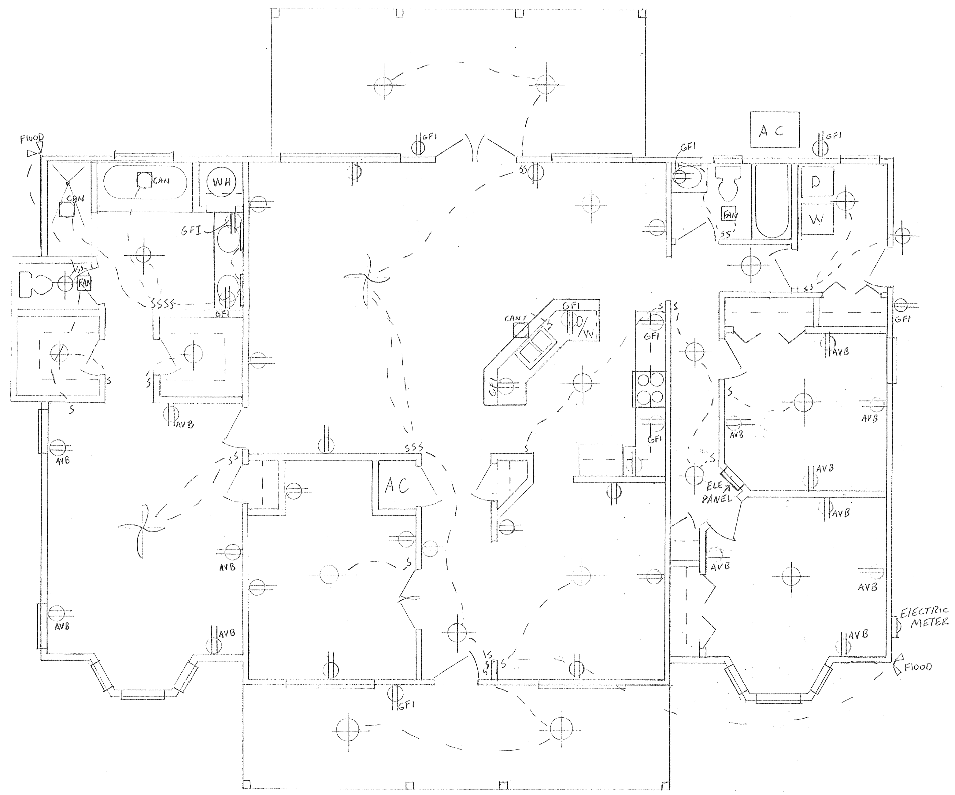
ELECTRICAL PLAN 1'-0" = 1/4"
