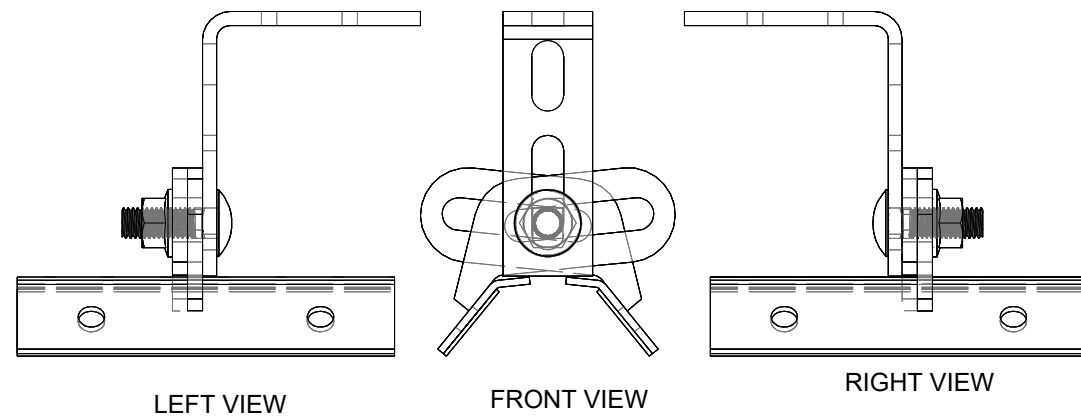
1 ATTACHMENT DETAILS S-02 SCALE: 3" = 1'-0"
