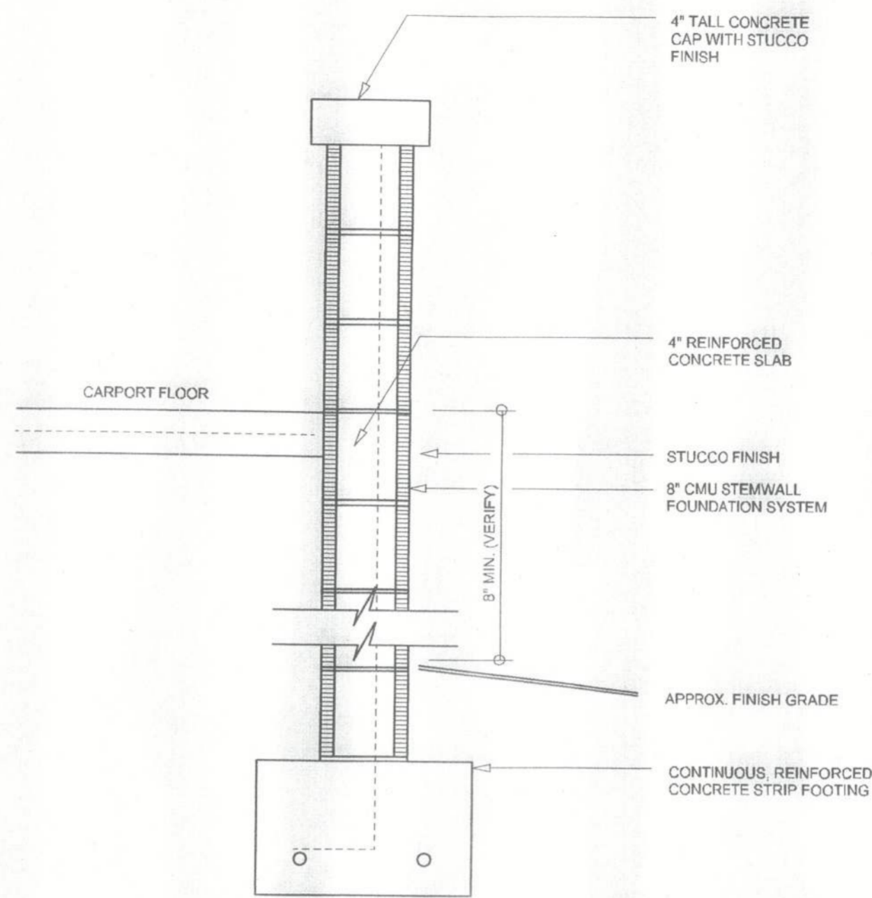
A-2 TYPICAL WALL SECTION SCALE: 1" = 1'-0"
