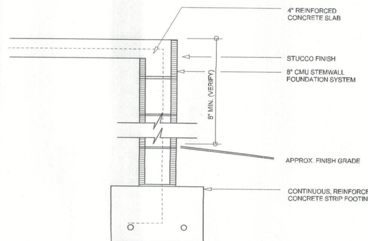
A-3 TYPICAL WALL SECTION SCALE: 1" = 1'-0"
