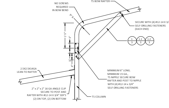
7A SIDE EXTENSION RAFTER/COLUMN DETAIL FOR EXTENSION RAFTER SPANS W \leq 12'-0" , IF THE KNEE BRACE ON THE OTHER END OF THE RAFTER IS PER DETAIL 1.1/2. FOR EXTENSION RAFTER SPANS W \leq 13'-0" , IF THE KNEE BRACE ON THE OTHER END OF THE RAFTER IS PER DETAIL 1.1/3. FOR EXTENSION RAFTER SPANS W < 15'-0" , IF THE KNEE BRACE ON THE OTHER END OF THE RAFTER IS PER DETAIL 1/3. SCALE: NTS
