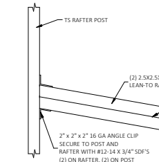
6C LEAN-TO RAFTER TO RAFTER COLUMN CONNECTION DETAIL FOR LEAN-TO RAFTER SPANS 16'-0" < W \leq 24'-0" , IF THE KNEE BRACE ON THE OTHER END OF THE RAFTER IS PER DETAIL 1.1/2 OR 1.2/3. FOR LEAN-TO RAFTER SPANS 18'-0" < W \leq 24'-0" , IF THE KNEE BRACE ON THE OTHER END OF THE RAFTER IS PER DETAIL 1.1/2 OR 1.1/3. FOR LEAN-TO RAFTER SPANS 19'-0" < W < 24'-0" , IF THE KNEE BRACE ON THE OTHER END OF THE RAFTER IS PER DETAIL 1/2 OR 1/3. SCALE: NTS
