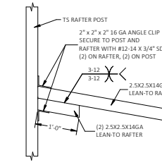
6B LEAN-TO RAFTER TO RAFTER COLUMN CONNECTION DETAIL FOR LEAN-TO RAFTER SPANS 12'-0" < W \leq 16'-0" , IF THE KNEE BRACE ON THE OTHER END OF THE RAFTER IS PER DETAIL 1.1/2 OR 1.2/3. FOR LEAN-TO RAFTER SPANS 13'-0" < W \leq 18'-0" , IF THE KNEE BRACE ON THE OTHER END OF THE RAFTER IS PER DETAIL 1.1/2 OR 1.1/3. FOR LEAN-TO RAFTER SPANS 15'-0" < W < 19'-0" , IF THE KNEE BRACE ON THE OTHER END OF THE RAFTER IS PER DETAIL 1/2 OR 1/3. SCALE: NTS
