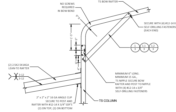
7C SIDE EXTENSION RAFTER/COLUMN DETAIL FOR EXTENSION RAFTER SPANS 16'-0" < W \leq 24'-0" , IF THE KNEE BRACE ON THE OTHER END OF THE RAFTER IS PER DETAIL 1.1/2. FOR EXTENSION RAFTER SPANS 18'-0" < W \leq 24'-0" , IF THE KNEE BRACE ON THE OTHER END OF THE RAFTER IS PER DETAIL 1.1/3. FOR EXTENSION RAFTER SPANS 19'-0" < W < 24'-0" , IF THE KNEE BRACE ON THE OTHER END OF THE RAFTER IS PER DETAIL 1/3. SCALE: NTS
