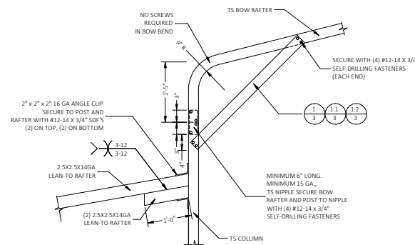
SIDE EXTENSION RAFTER/COLUMN DETAIL FOR EXTENSION RAFTER SPANS 12'-0" < W' <= 16'-0", IF THE KNEE BRACE ON THE OTHER END OF THE RAFTER IS PER DETAIL 1.2/3. FOR EXTENSION RAFTER SPANS 13'-0" < W' <= 18'-0", IF THE KNEE BRACE ON THE OTHER END OF THE RAFTER IS PER DETAIL 1.1/3. FOR EXTENSION RAFTER SPANS 15'-0" < W' <= 19'-0", IF THE KNEE BRACE ON THE OTHER END OF THE RAFTER IS PER DETAIL 1/3. SCALE: NTS
