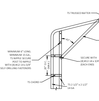
1B BOW EAVE RAFTER COLUMN CONNECTION DETAIL FOR HEIGHTS 16'-0" < TO ≤ 20'-0" SCALE: NTS
