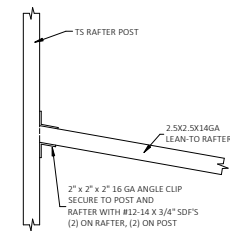
6A LEAN-TO RAFTER TO RAFTER COLUMN CONNECTION DETAIL FOR LEAN-TO RAFTER SPANS W \leq 12'-0" , IF THE KNEE BRACE ON THE OTHER END OF THE RAFTER IS PER DETAIL 1.1/2 OR 1.2/3. FOR LEAN-TO RAFTER SPANS W \leq 13'-0" , IF THE KNEE BRACE ON THE OTHER END OF THE RAFTER IS PER DETAIL 1.1/2 OR 1.1/3. FOR LEAN-TO RAFTER SPANS W \leq 15'-0" , IF THE KNEE BRACE ON THE OTHER END OF THE RAFTER IS PER DETAIL 1/2 OR 1/3. SCALE: NTS
