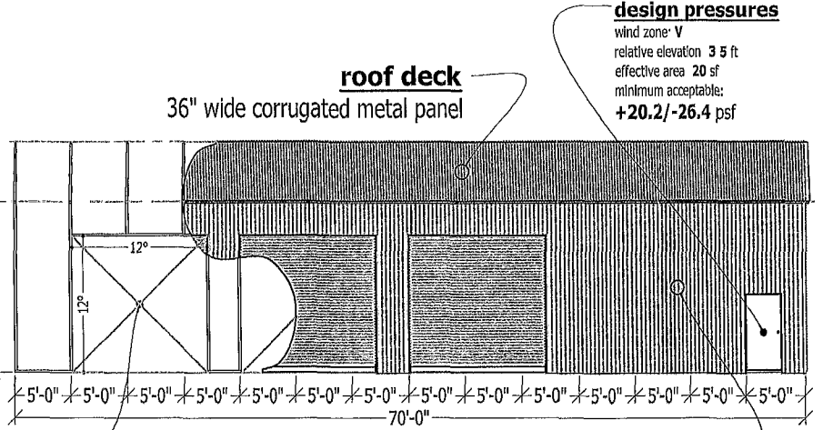
left side composite proportional scale
