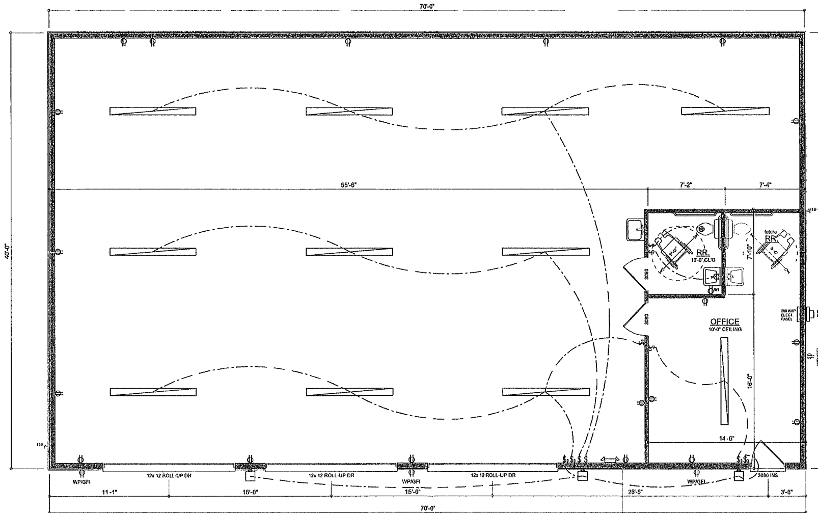
DIMENSIONED FLOOR PLAN & ELECTRICAL SCALE: 1/4" = 1'-0"
