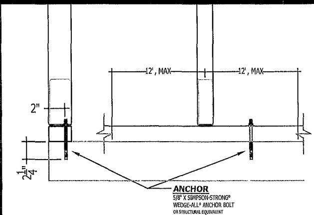
TYPE CA-1: DIRECT ANCHOR PROPORTIONAL SCALE
