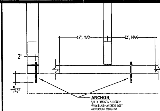
TYPE CA-1: DIRECT ANCHOR PROPORTIONAL SCALE
