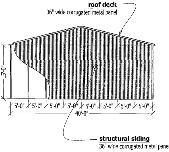
rear gable composite proportional scale
