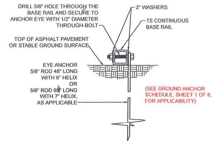
1D BASE RAIL DEEP ANCHORAGE
