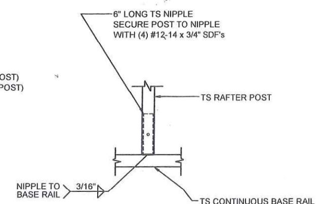
3 POST/BASE RAIL CONN. DETAIL
