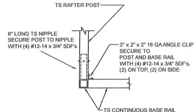
5 END POST/BASE RAIL CONN.
