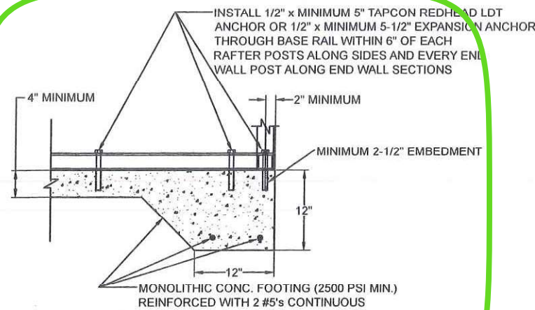
1A CONCRETE BASE RAIL ANCHORAGE
