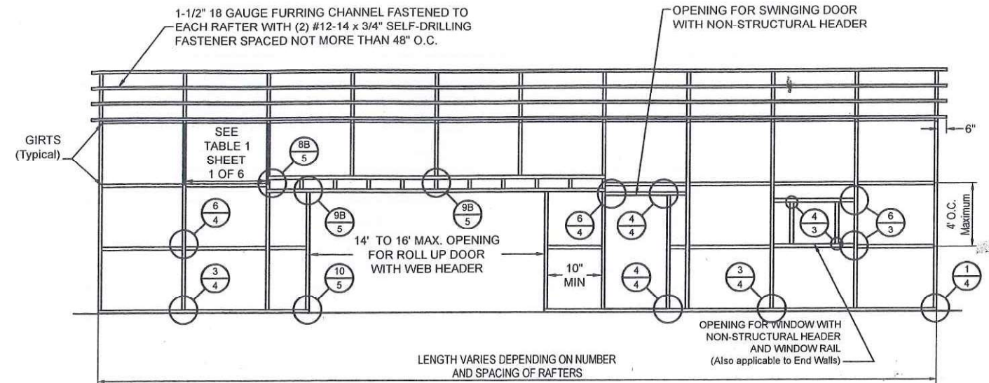
TYPICAL POST/RAFTER/GIRT FRAMING PLAN
