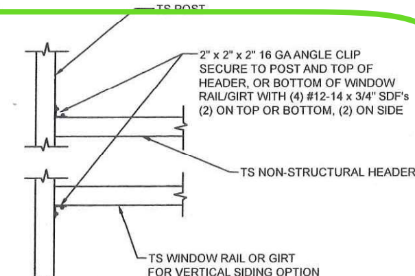
6 NON-STRUCTURAL HEADER, WINDOW RAIL, OR GIRT TO POST CONN. DETAIL
