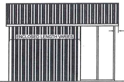
TYPICAL SIDE ELEVATION
