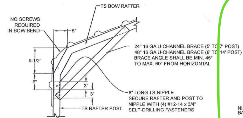
2B BOW RAFTER/POST DETAIL
