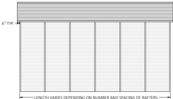
TYPICAL SIDE ELEVATION - EXTRA SIDE PANELS
