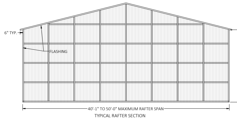
TYPICAL END ELEVATION VERTICAL ROOF/SIDING OPTION
