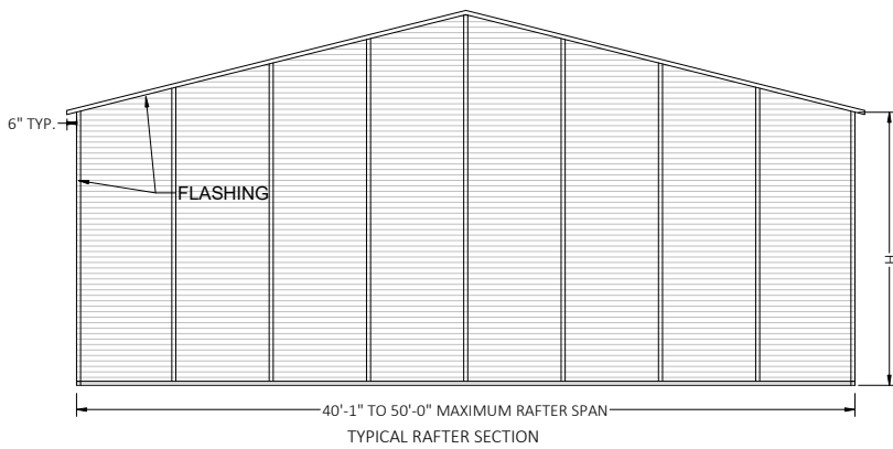
TYPICAL END ELEVATION EXTRA SIDE PANELS
