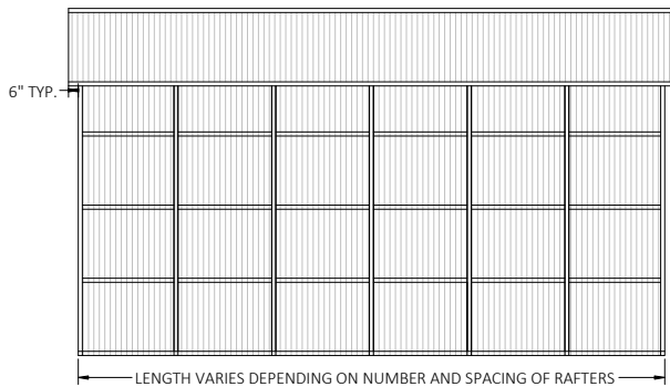
TYPICAL SIDE ELEVATION - VERTICAL ROOF/SIDING OPTION
