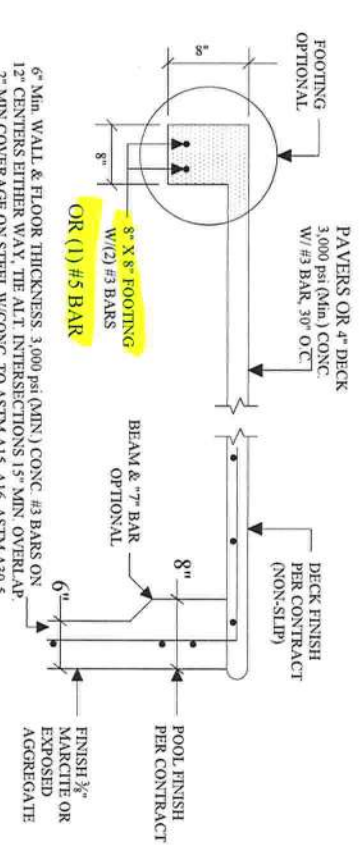
POOL/SPA, DECK, BEAM, WALL, FLOOR N.T.S.
