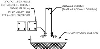
2C ENDWALL COLUMN/BASE RAIL CONNECTION DETAIL SCALE: NTS
