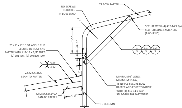
FOR EXTENSION RAFTER SPANS 12'-0" < W' <= 16'-0", IF THE KNEE BRACE ON THE OTHER END OF THE RAFTER IS PER DETAIL 1.2/3. FOR EXTENSION RAFTER SPANS 13'-0" < W' <= 18'-0", IF THE KNEE BRACE ON THE OTHER END OF THE RAFTER IS PER DETAIL 1.1/3. FOR EXTENSION RAFTER SPANS 15'-0" < W' <= 19'-0", IF THE KNEE BRACE ON THE OTHER END OF THE RAFTER IS PER DETAIL 1/3. SCALE: NTS
