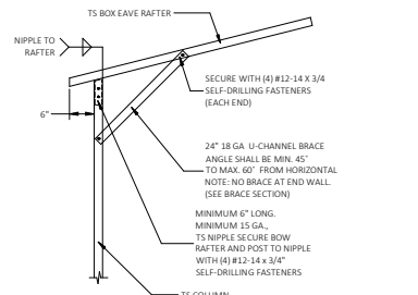
1.2 BOX EAVE RAFTER COLUMN CONNECTION DETAIL FOR HEIGHTS ≤ 12'-0" SCALE: NTS
