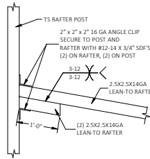
RAFTER COLUMN CONNECTION DETAIL KNEE BRACE ON THE OTHER END OF THE RAFTER IS PER DETAIL 1.2/2 OR 1.2/3. KNEE BRACE ON THE OTHER END OF THE RAFTER IS PER DETAIL 1.1/2 OR 1.1/3. KNEE BRACE ON THE OTHER END OF THE RAFTER IS PER DETAIL 1/2 OR 1/3. SCALE: NTS
