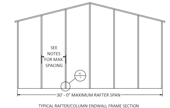
TYPICAL RAFTER/COLUMN ENDWALL FRAME SECTION
