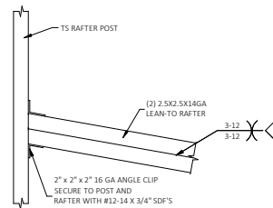
RAFTER COLUMN CONNECTION DETAIL KNEE BRACE ON THE OTHER END OF THE RAFTER IS PER DETAIL 1.2/2 OR 1.2/3. KNEE BRACE ON THE OTHER END OF THE RAFTER IS PER DETAIL 1.1/2 OR 1.1/3. KNEE BRACE ON THE OTHER END OF THE RAFTER IS PER DETAIL 1/2 OR 1/3. SCALE: NTS
