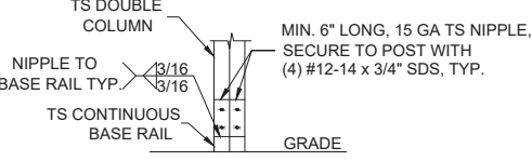
2B POST/BASE RAIL CONNECTION SCALE: NTS
