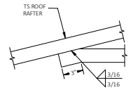
COLLAR-TIE CONNECTION SCALE: NTS
