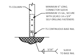
2 RAFTER POST/BASE RAIL CONNECTION DETAIL SCALE: NTS
