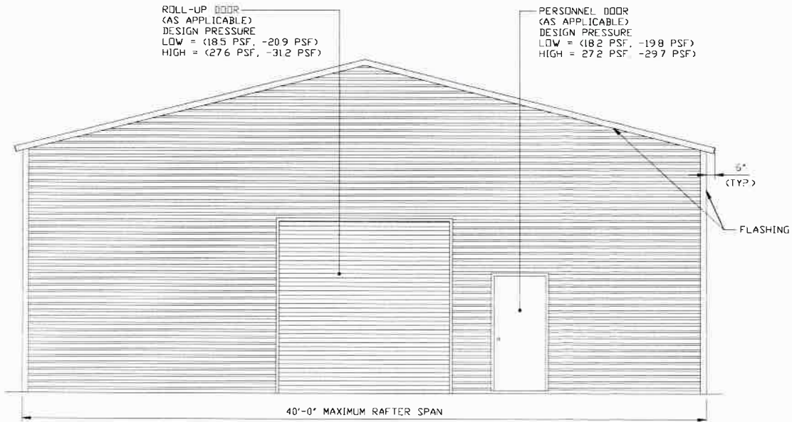
TYPICAL END ELEVATION-HORIZONTAL ROOF SCALE: 1/8" = 1'-0"
