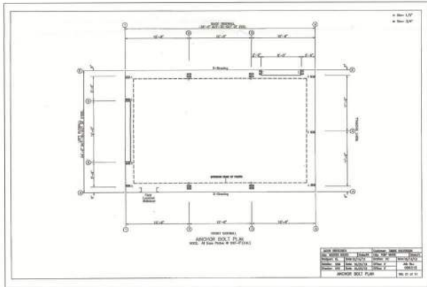
BUILDING OVERLAY OF FOUNDATION 1"=8'
