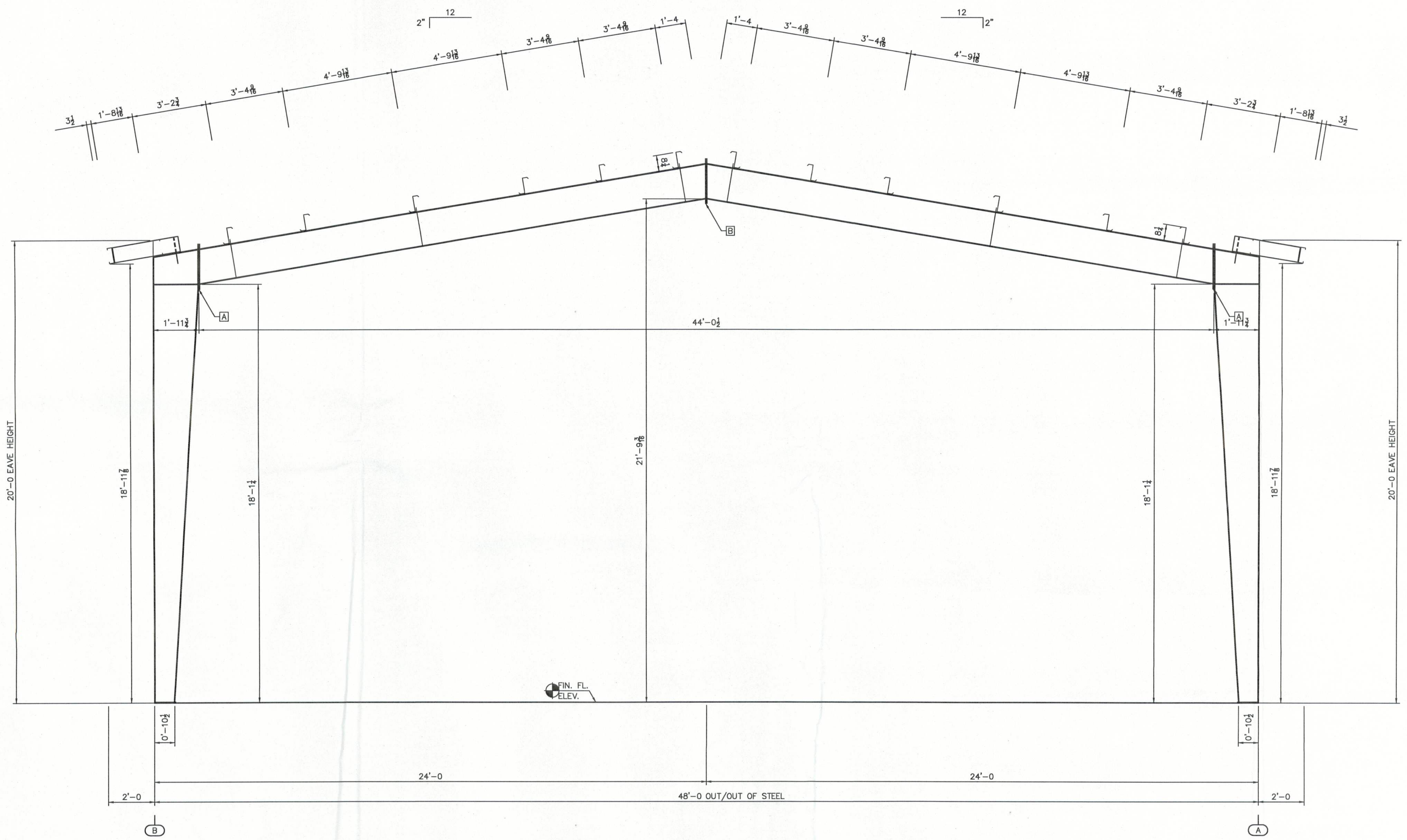
CROSS SECTION AT GRID LINE "3"
