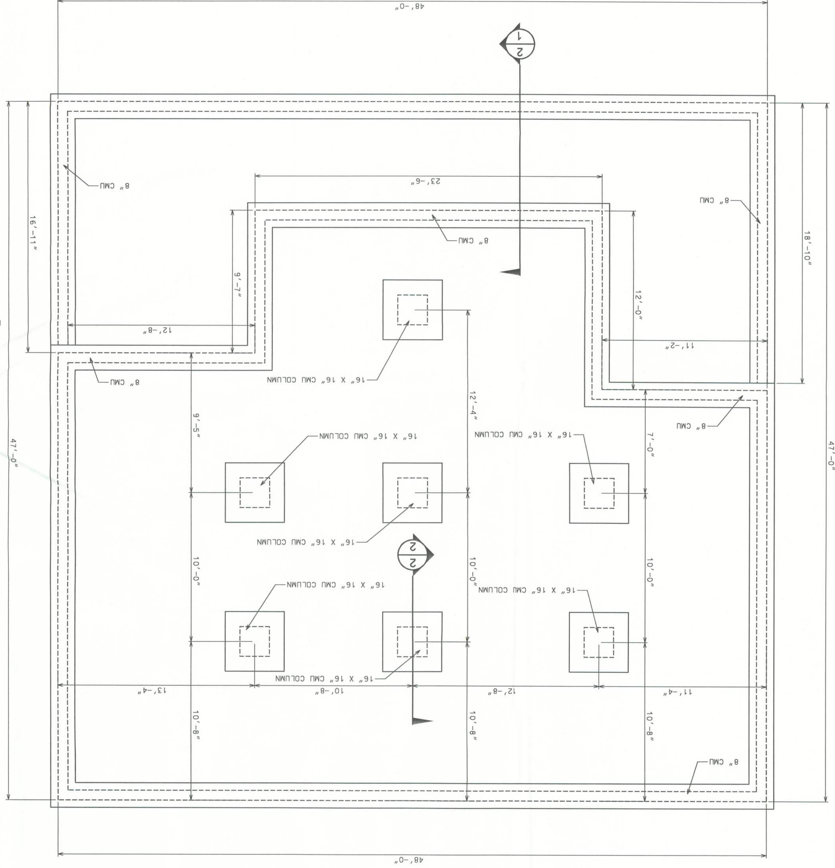
FOUNDATION LAYOUT
