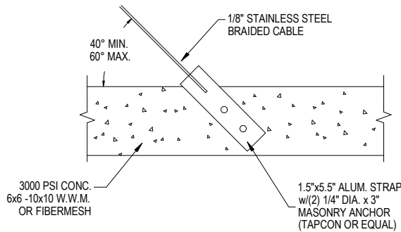
DETAIL "I-1" CABLE CONNECTION AT FOUNDATION SCALE: NTS
