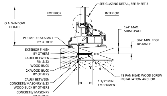
B 4 VERTICAL SECTION SILL - 2X WOOD BUCK NAIL FIN
