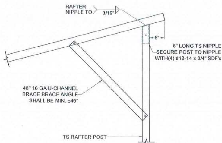
14 FREE-STANDING LEAN-TO TRUSSED Not To Scale
