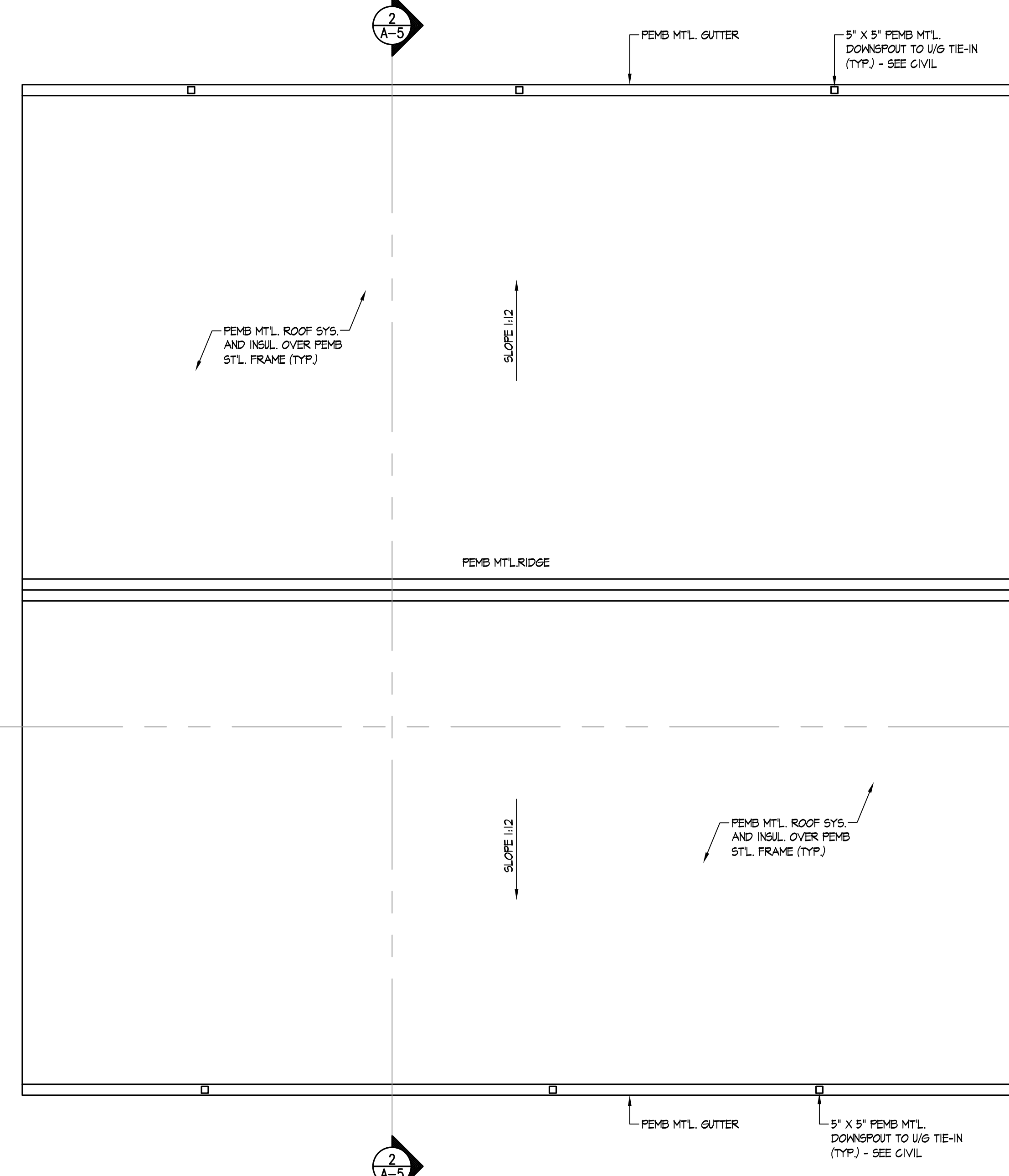
ROOF PLAN 3/16" = 1'-0"
