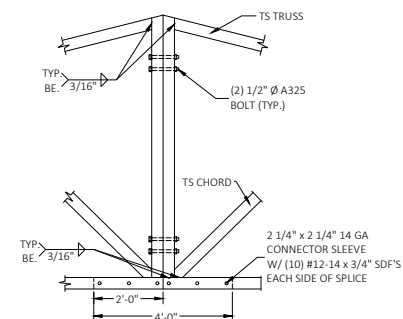
5 SPLICE CONNECTION SCALE: NTS
