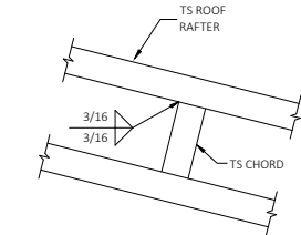
3 RAFTER TO CHORD CONNECTION SCALE: NTS
