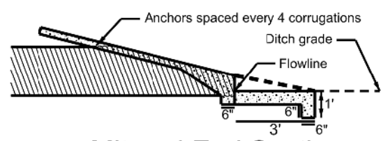
Mitered End Section Detail
