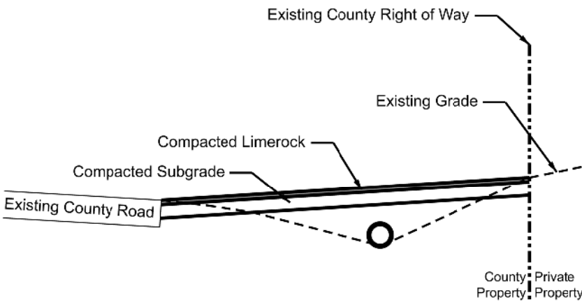
Driveway Connection Section A - A'
