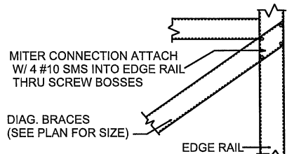
DIAGONAL ROOF BRACE DETAIL PLAN VIEW
