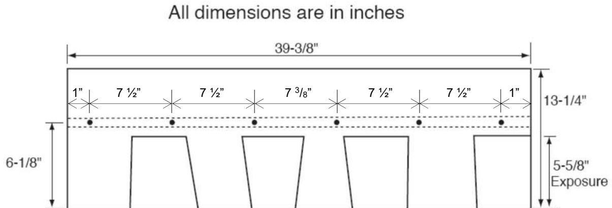
FIG. 1 FASTENING PATTERN
